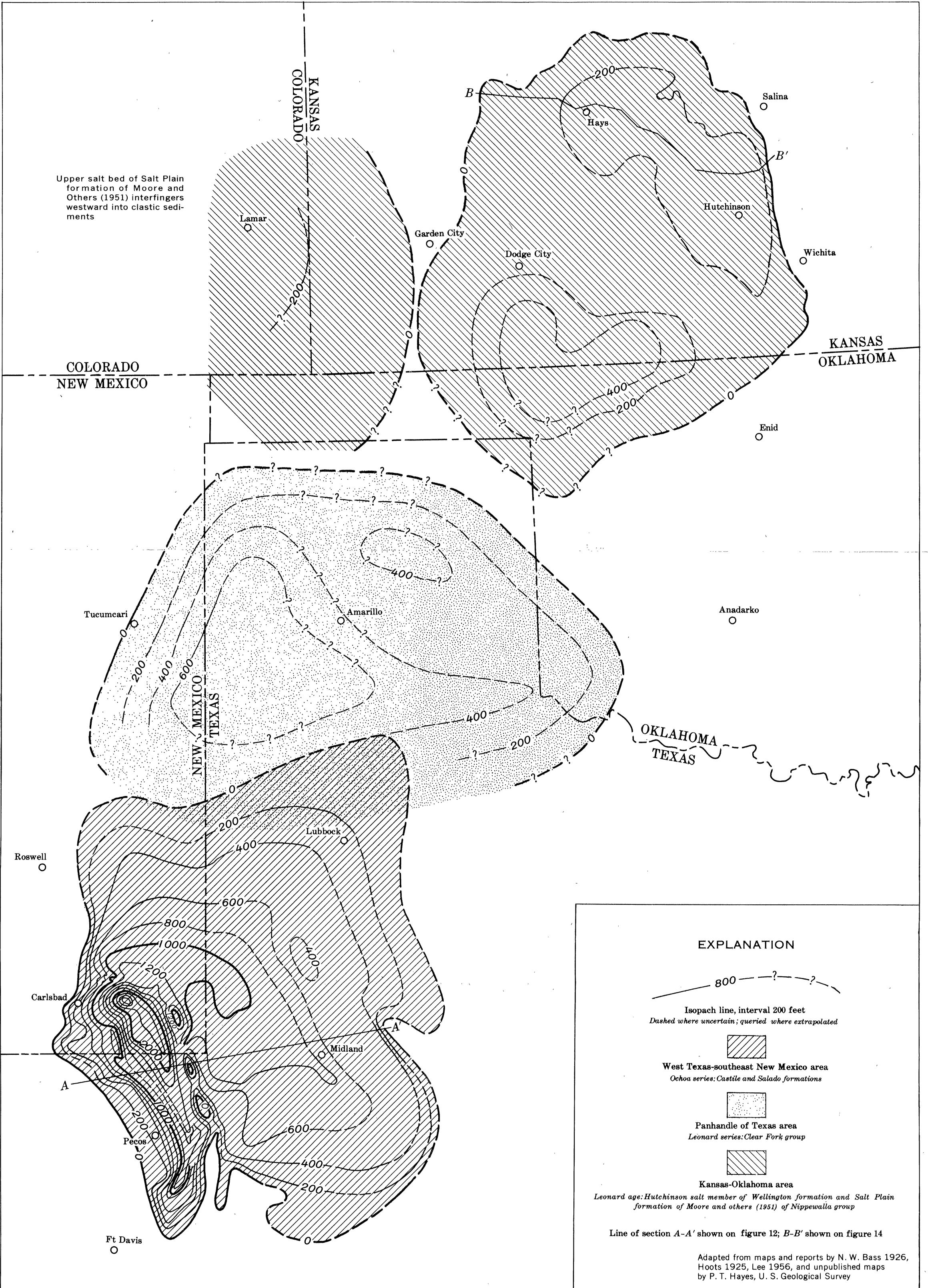
MAP SHOWING AGGREGATE THICKNESS OF SALT IN PERMIAN BASIN OF KANSAS, OKLAHOMA, TEXAS, AND NEW MEXICO
