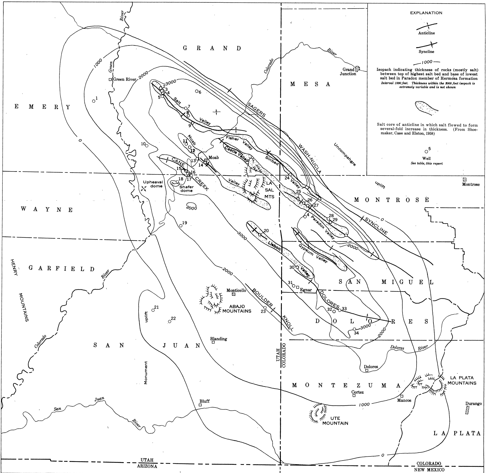
MAP OF PARADOX BASIN AREA SHOWING THICKNESS OF SALT-BEARING ROCKS OF PARADOX MEMBER OF HERMOSA FORMATION, AND THEIR RELATION TO MAJOR STRUCTURAL AND PHYSIOGRAPHIC FEATURES
