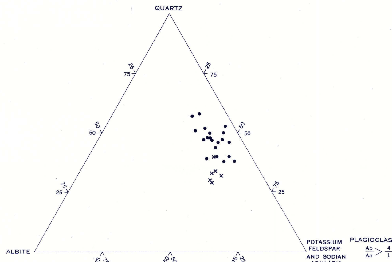
F. BOKAN MOUNTAIN GRANITE × Represents specimens from the Ross-Adams mine area
