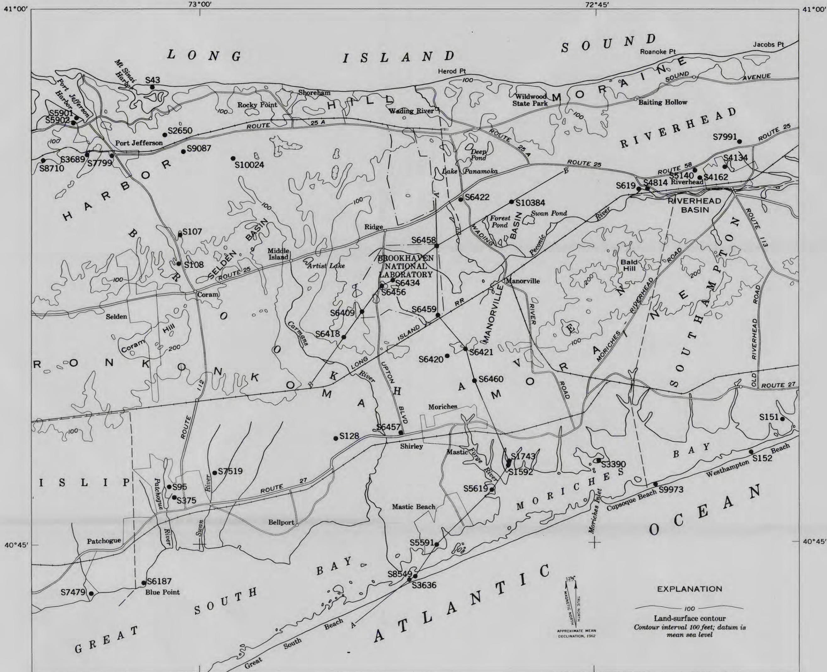
MAP OF CENTRAL SUFFOLK COUNTY, NEW YORK, SHOWING MAJOR TOPOGRAPHIC FEATURES AND LOCATION OF WELLS AND GEOLOGIC SECTIONS
