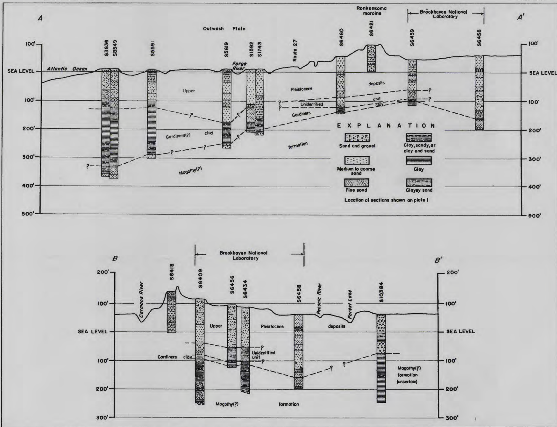
GEOLOGIC SECTIONS A-A' AND B-B', SUFFOLK COUNTY, NEW YORK
