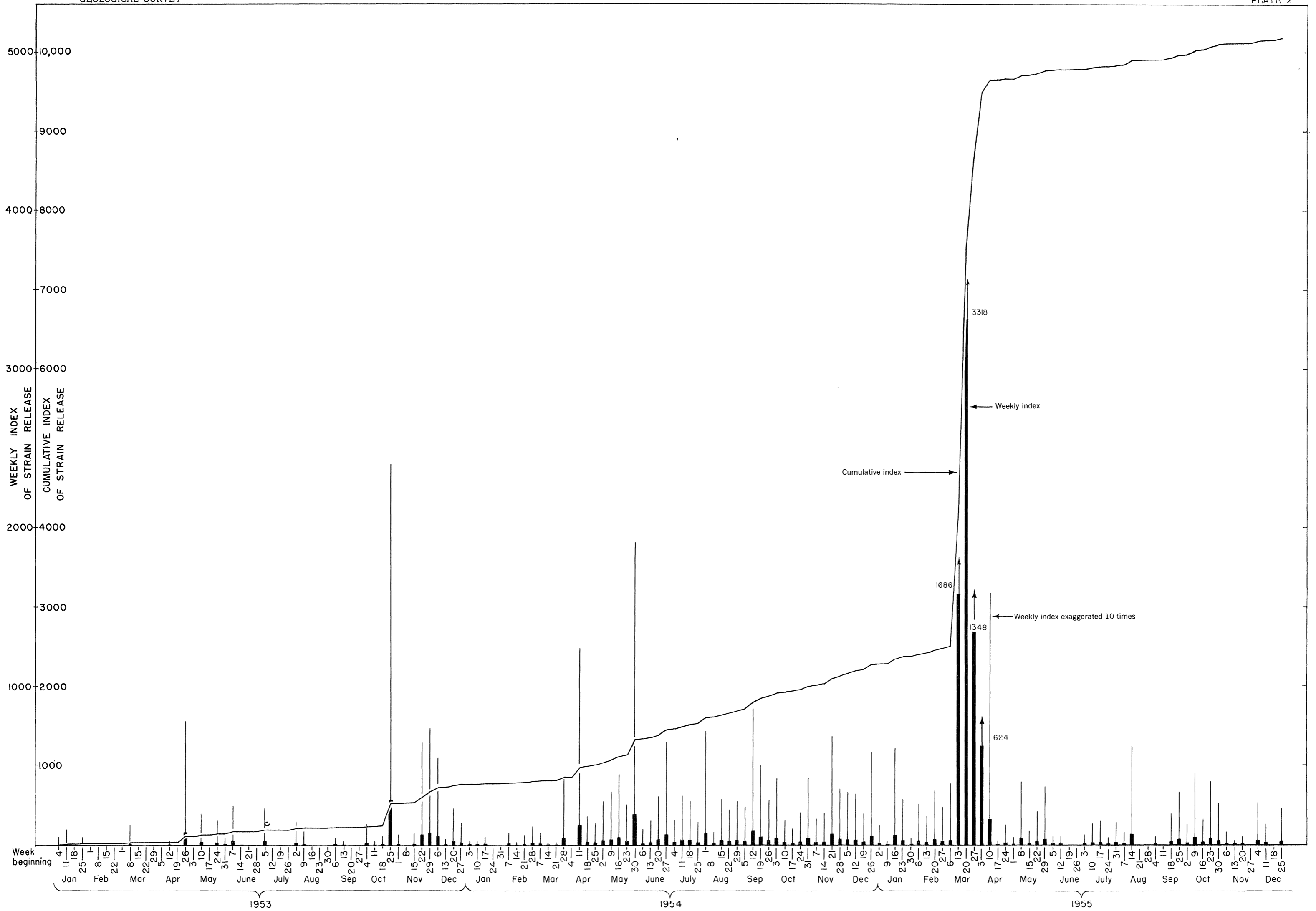
KILAUEA SUMMIT STRAIN-RELEASE INDEX FOR 1953 THROUGH 1955
