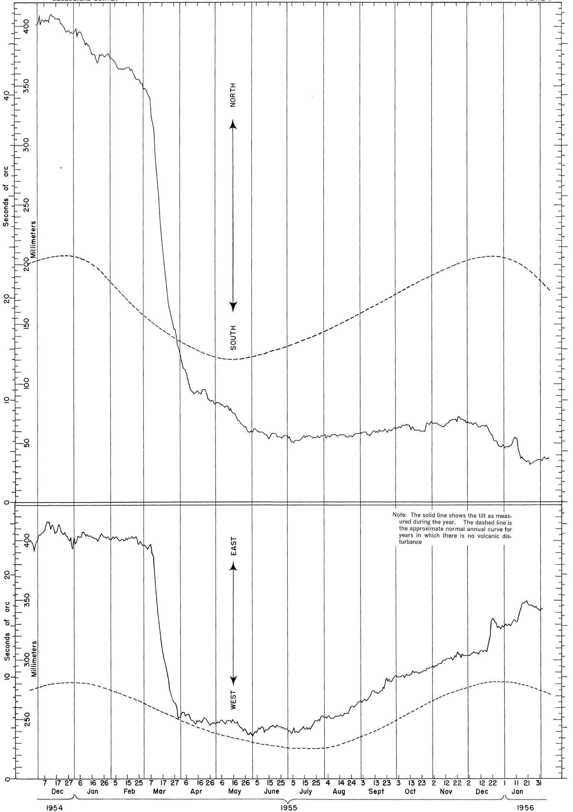
1954 1955 1956 GRAPH SHOWING TILTING OF THE GROUND SURFACE AT THE WHITNEY LABORATORY OF SEISMOLOGY, ON THE NORTHEAST RIM OF KILAUEA CALDERA, DURING 1955
