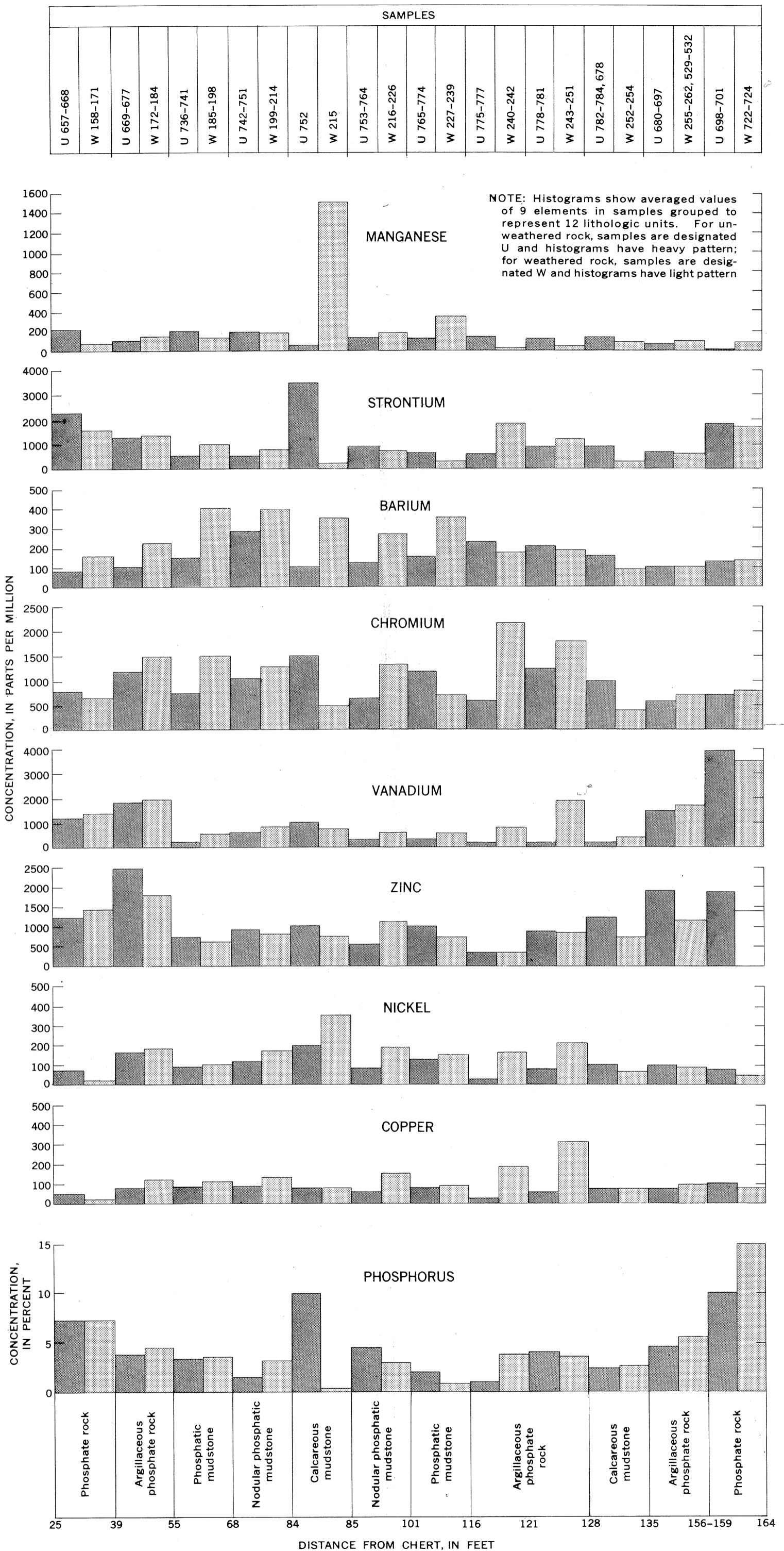
COMPARISON OF PARTIAL CHEMICAL COMPOSITION OF FRESH ROCK AND WEATHERED ROCK FROM THE MEADE PEAK PHOSPHATIC SHALE MEMBER OF THE PHOSPHORIA FORMATION NEAR GEORGETOWN IN SOUTHEASTERN IDAHO
