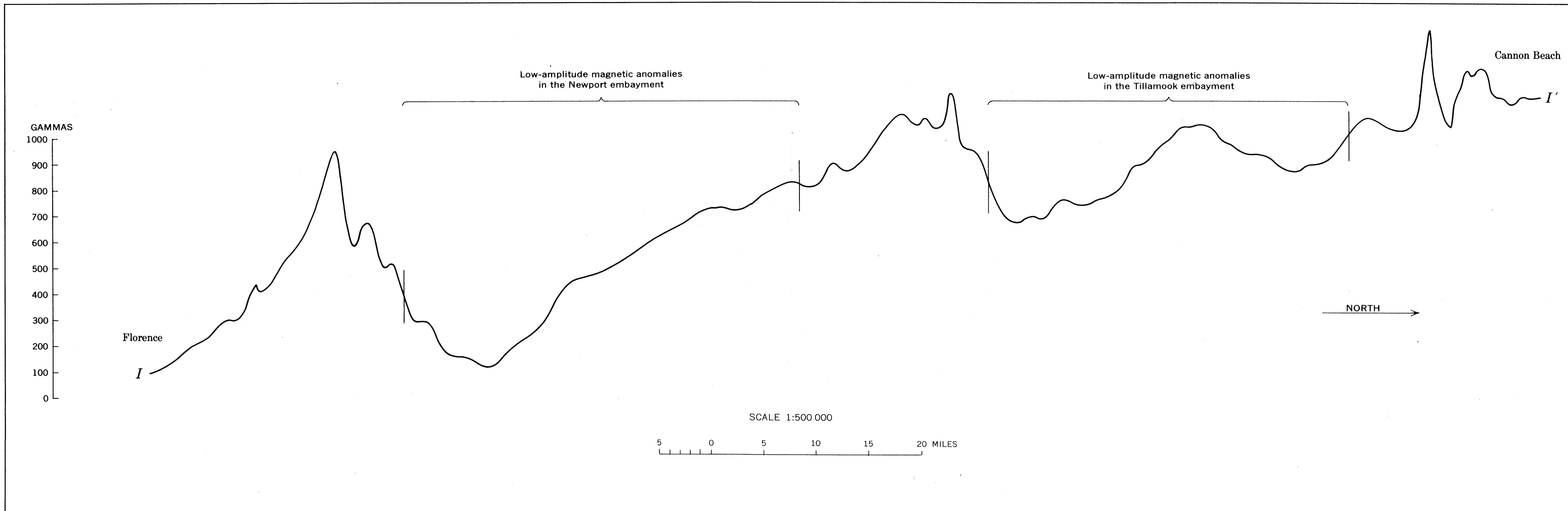
RECONNAISSANCE AEROMAGNETIC PROFILE ALONG THE OREGON COAST FROM FLORENCE TO CANNON BEACH
