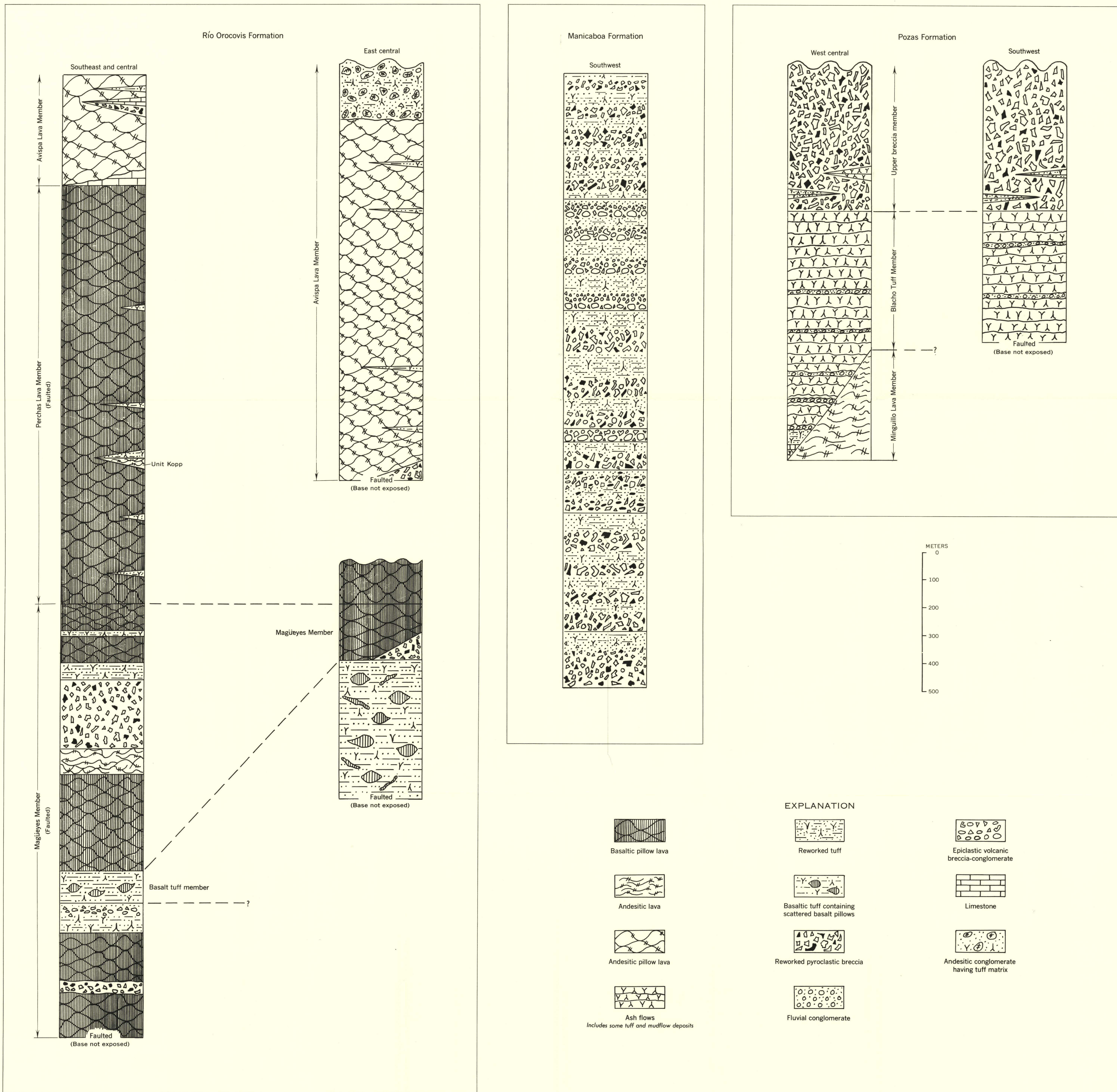
COMPOSITE COLUMNAR SECTIONS OF UPPER CRETACEOUS FORMATIONS IN THE CIALES QUADRANGLE, PUERTO RICO
