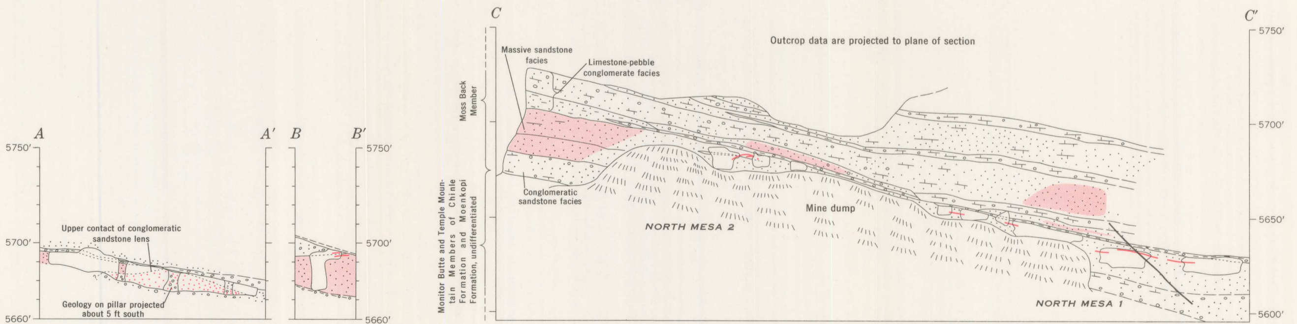
GEOLOGIC MAP AND SECTIONS OF THE NORTH MESA 1, 2, AND 5 MINES, TEMPLE MOUNTAIN DISTRICT, EMERY COUNTY, UTAH
