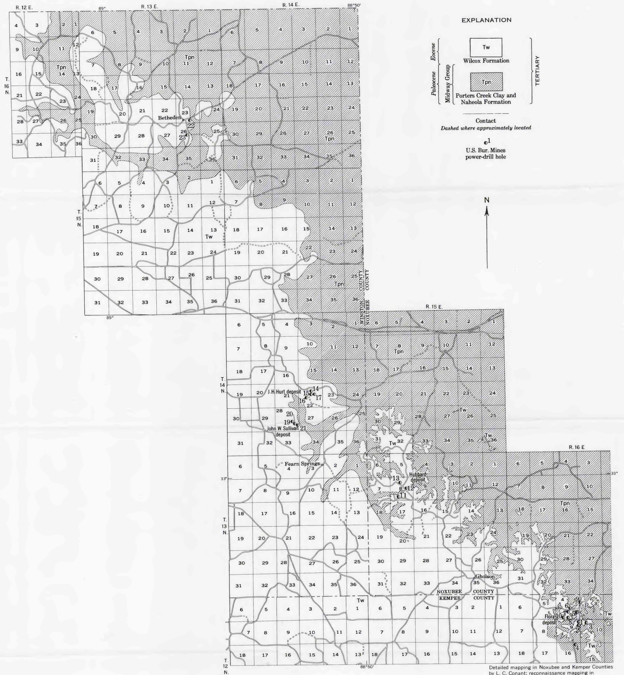
GEOLOGIC MAP OF THE WINSTON-NOXUBEE-KEMPER DISTRICT, MISSISSIPPI SHOWING LOCATION OF DRILL HOLES
