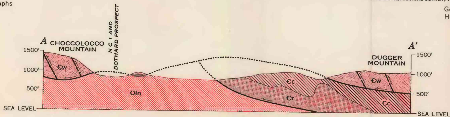
GEOLOGIC MAP AND SECTION OF THE NANCES CREEK BAUXITE AREA, CALHOUN COUNTY, ALABAMA
