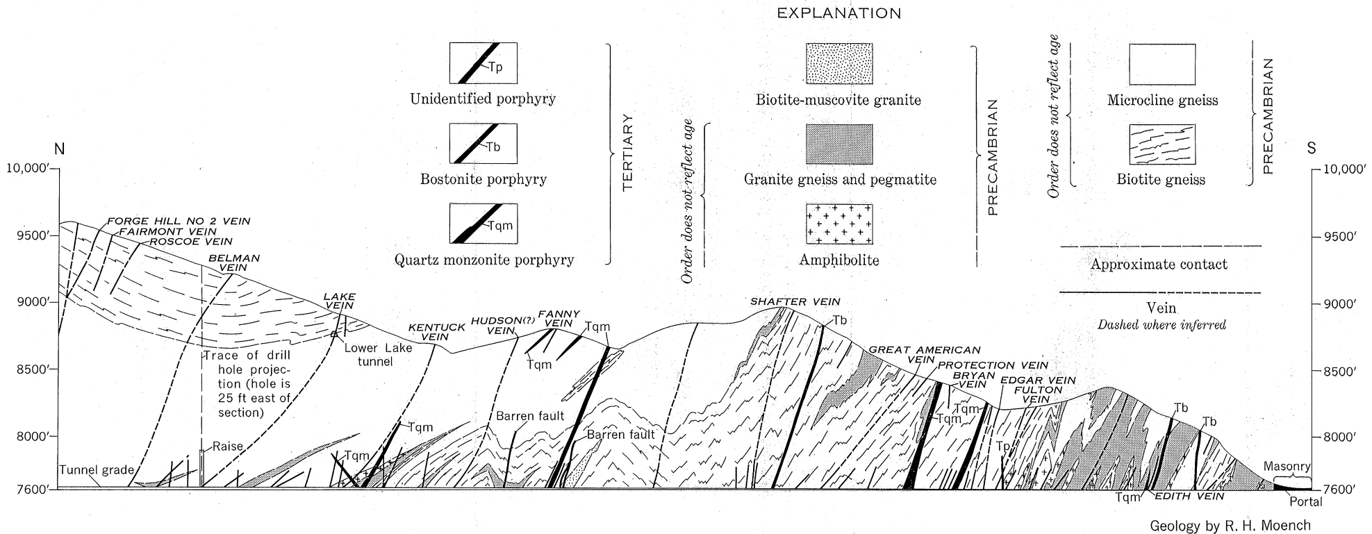
GEOLOGIC SECTION ALONG THE BIG FIVE TUNNEL, IDAHO SPRINGS DISTRICT, COLORADO
