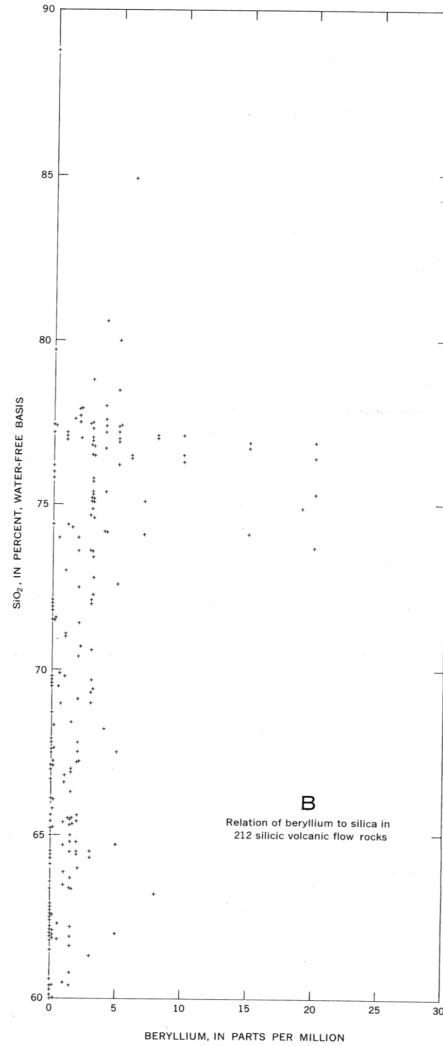
SCATTER DIAGRAMS SHOWING RELATION OF BERYLLIUM TO SILICA IN VOLCANIC ROCKS: A, TUFFS; B, FLOW ROCKS; C, GLASSY ROCKS
