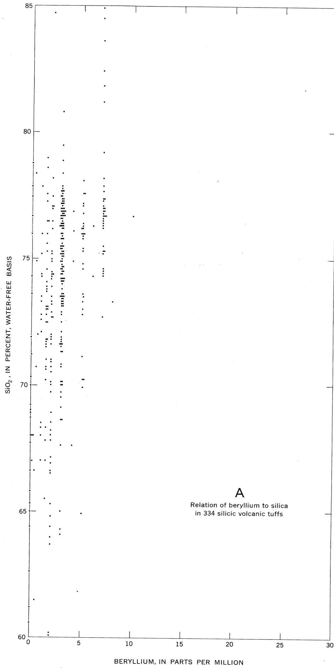
SCATTER DIAGRAMS SHOWING RELATION OF BERYLLIUM TO SILICA IN VOLCANIC ROCKS: A, TUFFS; B, FLOW ROCKS; C, GLASSY ROCKS
