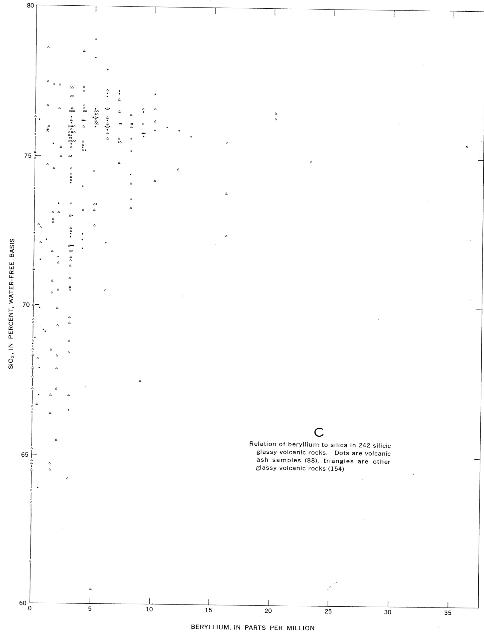
SCATTER DIAGRAMS SHOWING RELATION OF BERYLLIUM TO SILICA IN VOLCANIC ROCKS: A, TUFFS; B, FLOW ROCKS; C, GLASSY ROCKS
