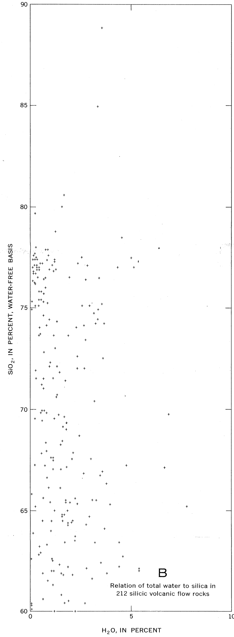
SCATTER DIAGRAMS SHOWING RELATION OF TOTAL WATER TO SILICA IN VOLCANIC ROCKS: A, TUFFS; B, FLOW ROCKS; C, GLASSY ROCKS
