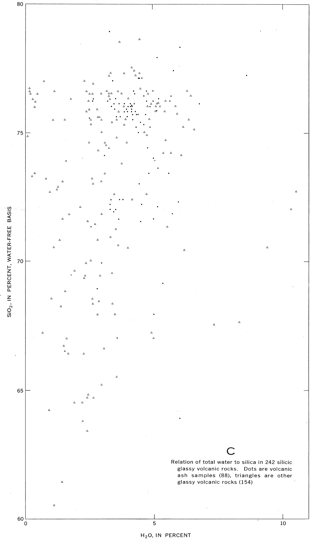
SCATTER DIAGRAMS SHOWING RELATION OF TOTAL WATER TO SILICA IN VOLCANIC ROCKS: A, TUFFS; B, FLOW ROCKS; C, GLASSY ROCKS
