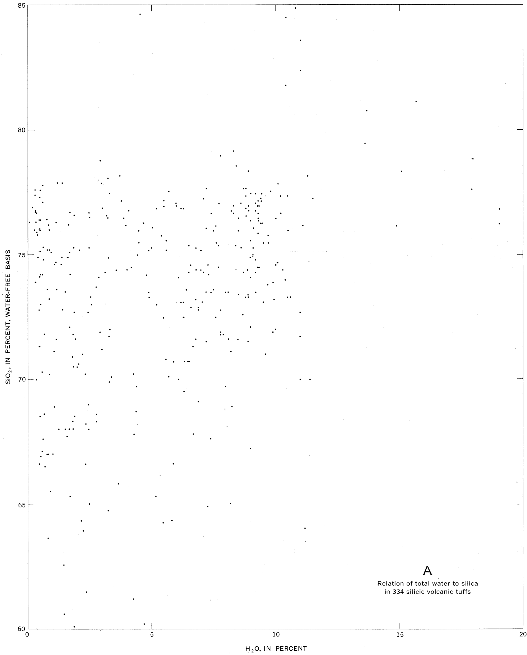
SCATTER DIAGRAMS SHOWING RELATION OF TOTAL WATER TO SILICA IN VOLCANIC ROCKS: A, TUFFS; B, FLOW ROCKS; C, GLASSY ROCKS
