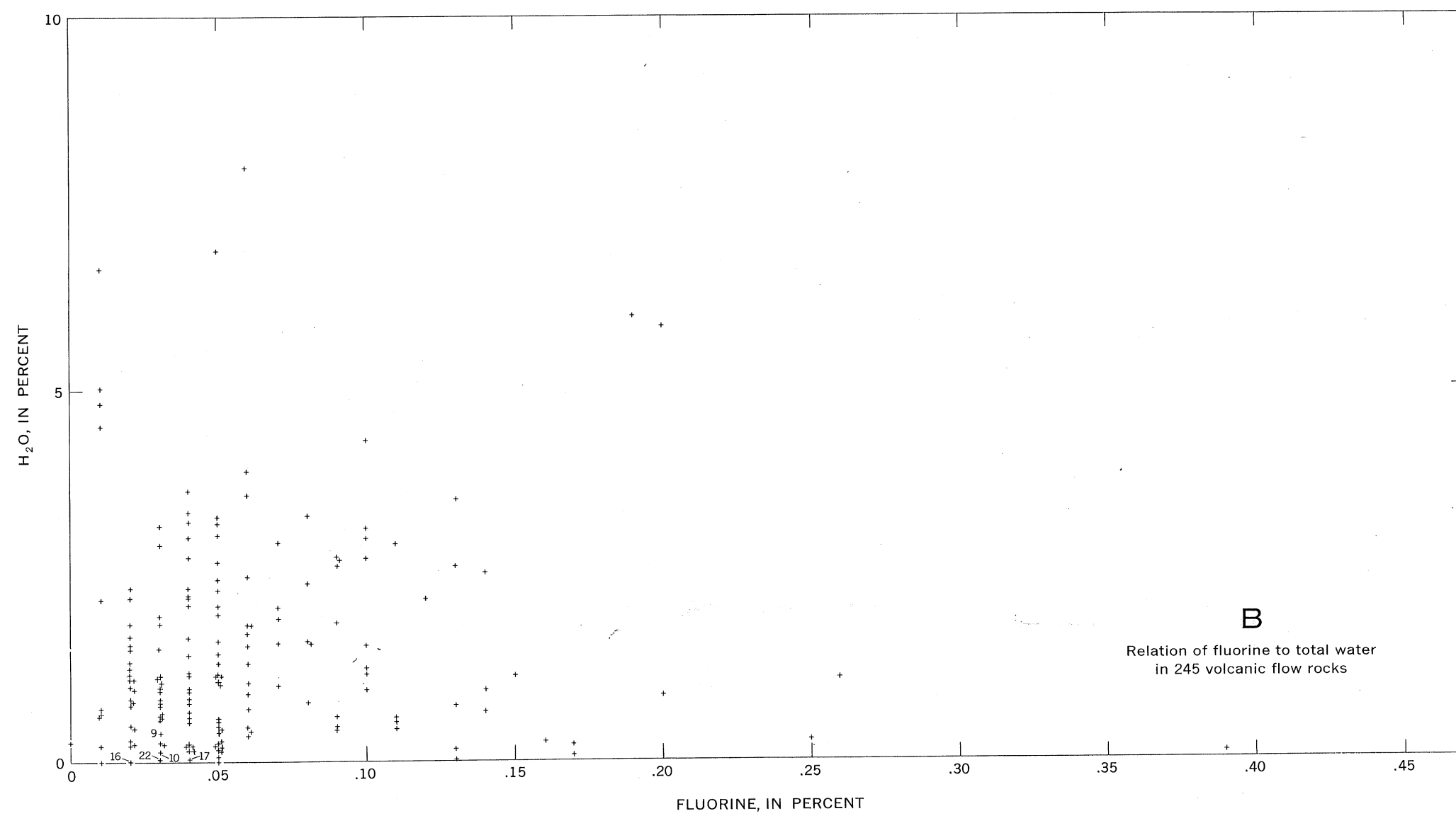
SCATTER DIAGRAMS SHOWING RELATION OF FLUORINE TO TOTAL WATER IN VOLCANIC ROCKS: A, TUFFS; B, FLOW ROCKS; C, GLASSY ROCKS
