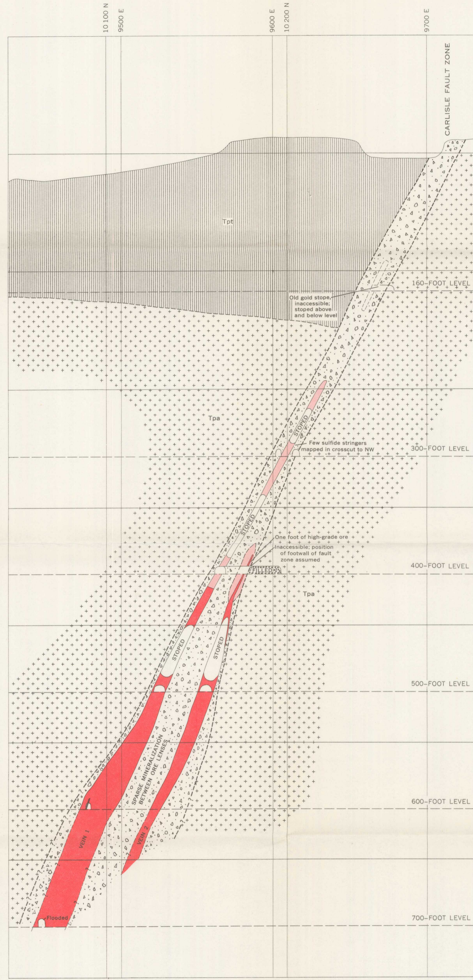
SECTION B-B'
