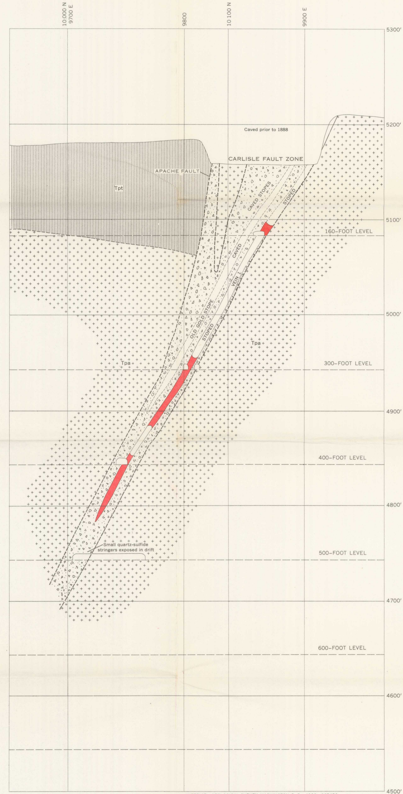
SECTION C-C'
