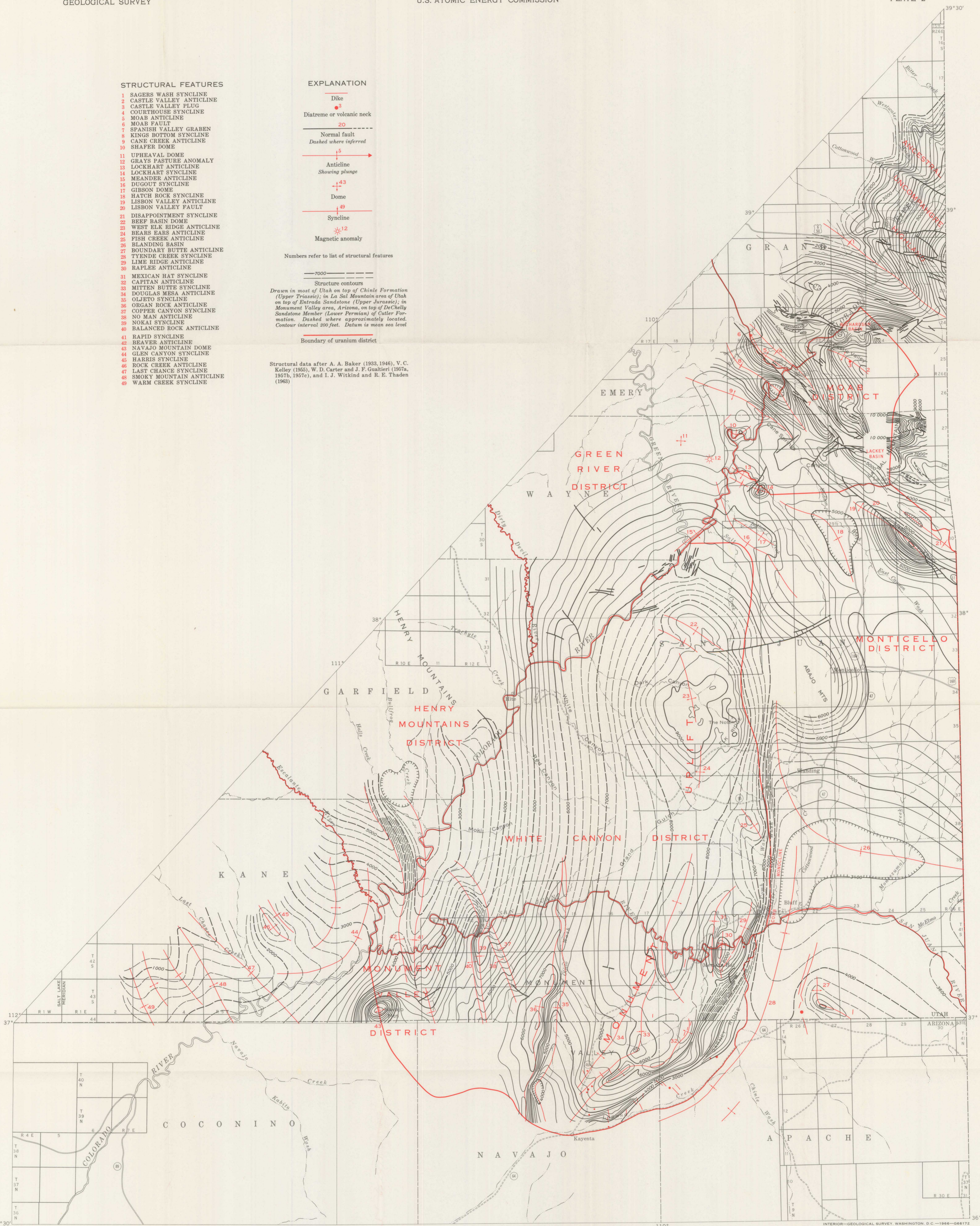
TECTONIC MAP OF THE MOAB, MONTICELLO, WHITE CANYON, AND MONUMENT VALLEY DISTRICTS, UTAH AND ARIZONA
