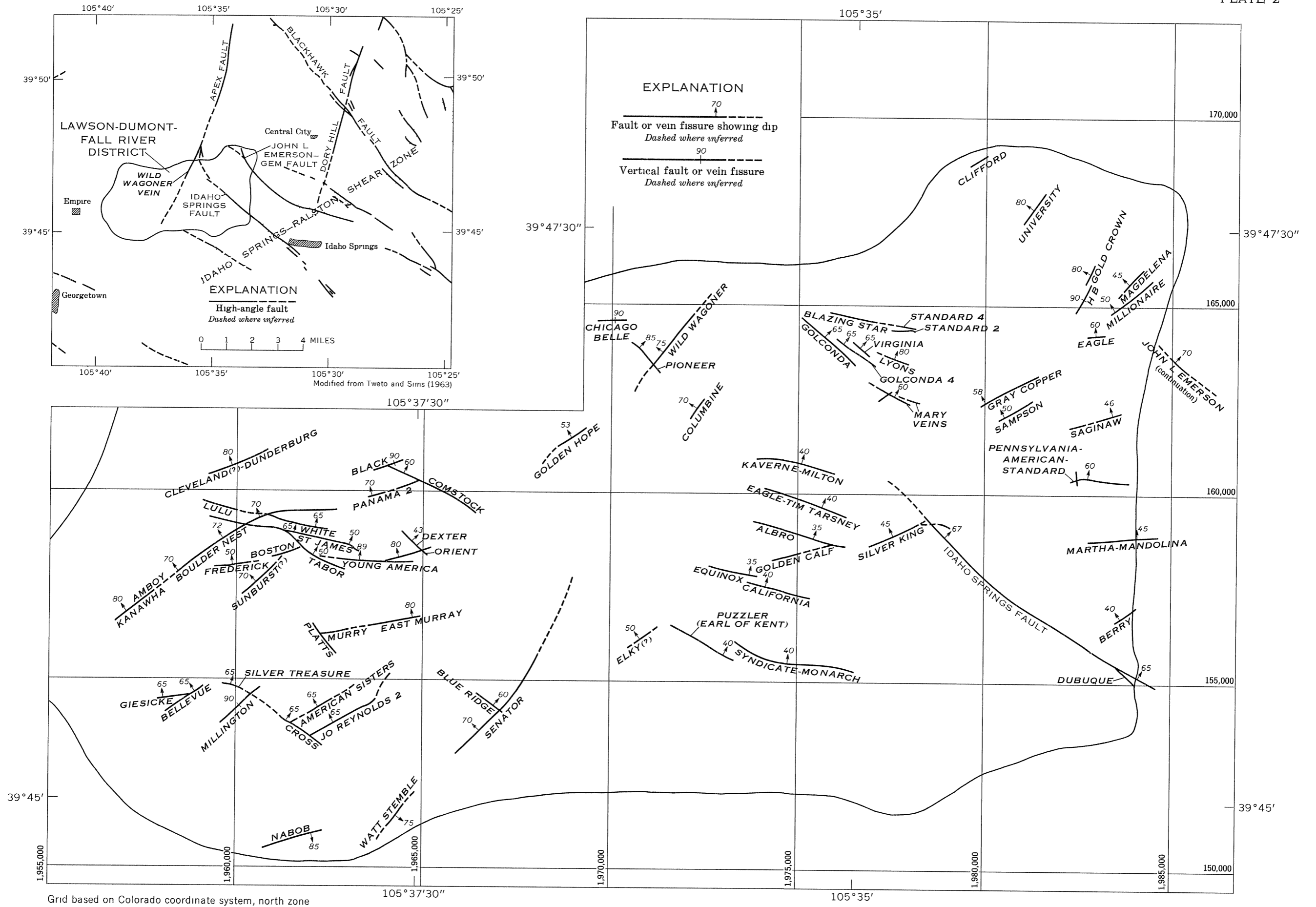
MAP SHOWING MAJOR FAULTS (VEINS) OF THE LAWSON-DUMONT-FALL RIVER DISTRICT, CLEAR CREEK COUNTY COLORADO, PROJECTED TO A HORIZONTAL PLANE HAVING AN ELEVATION OF 8,000 FEET
