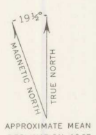
MAPS SHOWING ROCK TYPES AND STRUCTURAL FEATURES (A) AND ROCK TYPES, SAMPLE LOCATIONS AND MINERAL COMPOSITIONS (B) IN THE MOXIE PLUTON, GREENVILLE QUADRANGLE, MAINE
