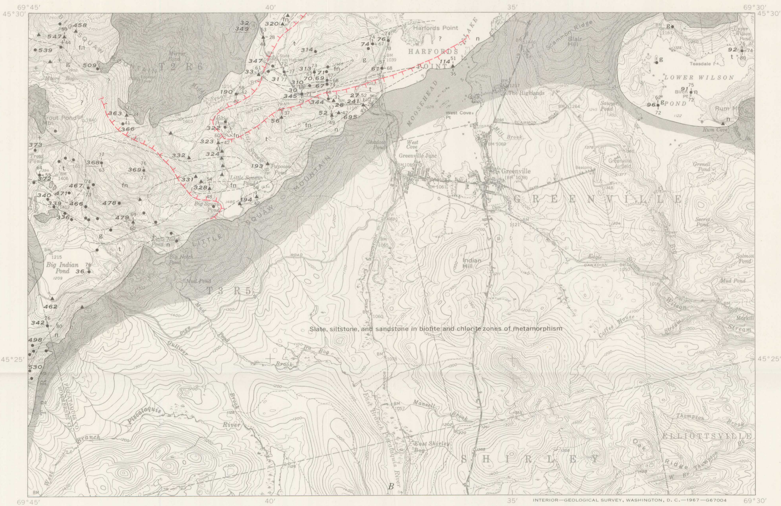
MAPS SHOWING ROCK TYPES AND STRUCTURAL FEATURES (A) AND ROCK TYPES, SAMPLE LOCATIONS AND MINERAL COMPOSITIONS (B) IN THE MOXIE PLUTON, GREENVILLE QUADRANGLE, MAINE
