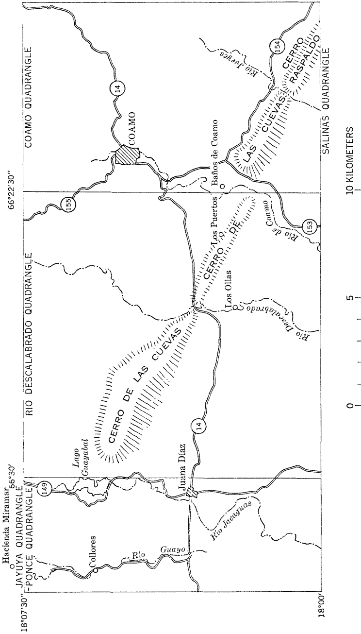
FIGURE 5.—Index map of central-southern Puerto Rico showing localities referred to in text.
