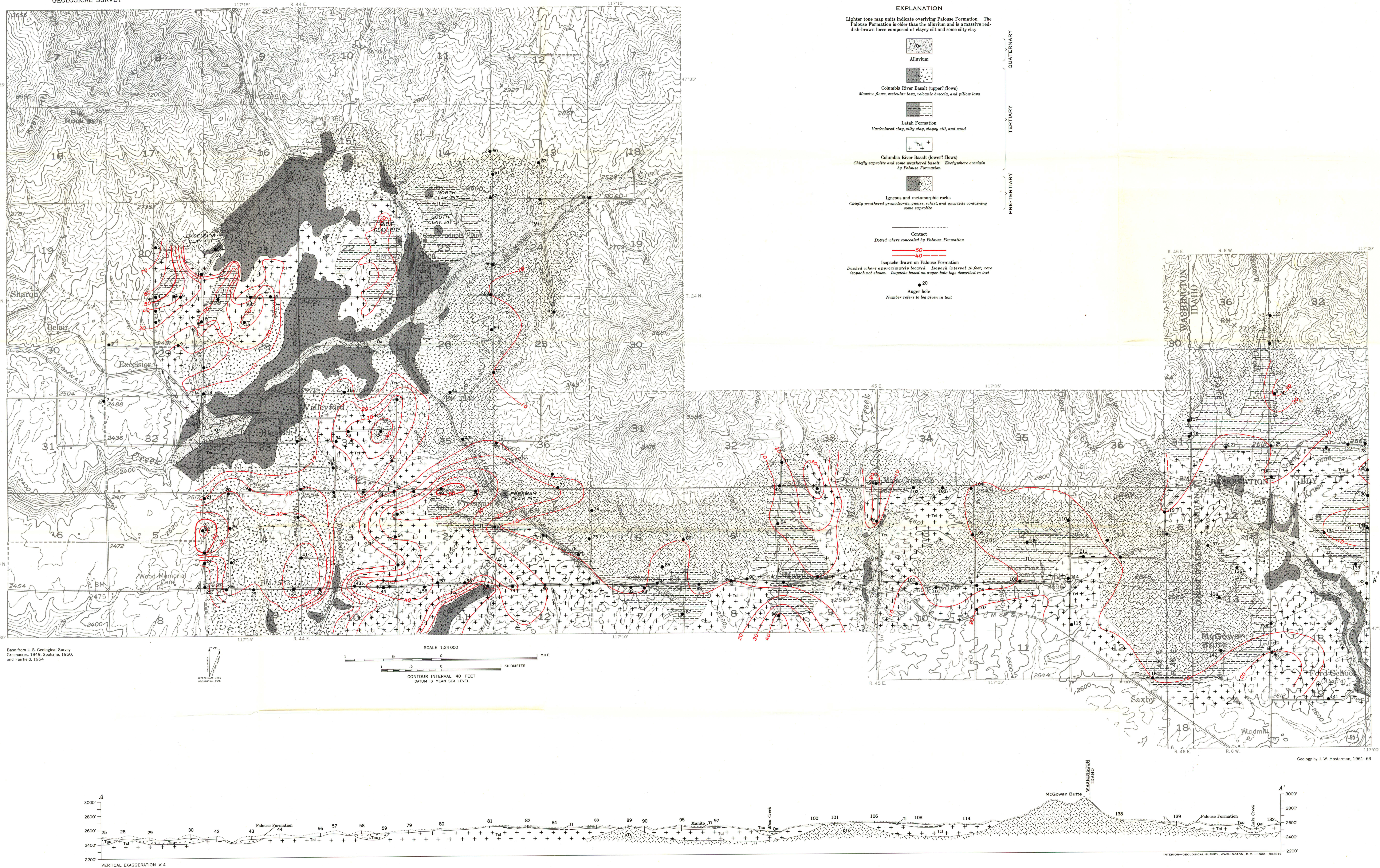
PRE-PALOUSE GEOLOGIC MAP AND SECTION, INCLUDING QUATERNARY ALLUVIUM, OF THE MICA-MANITO-SAXBY AREA, WASHINGTON-IDAHO
