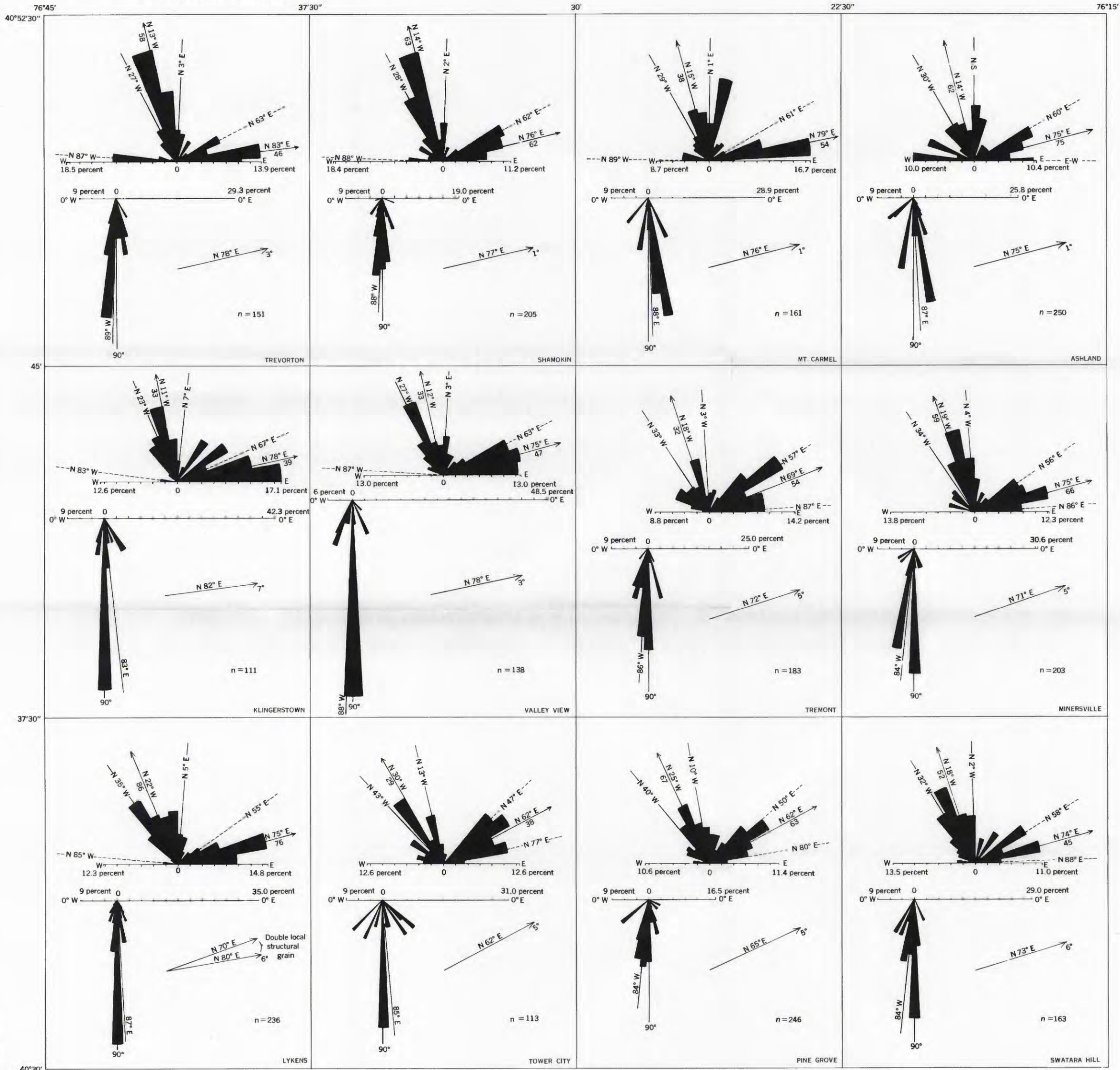
DIAGRAMS SHOWING RELATIONS OF JOINTS, STRUCTURAL GRAIN, AND PLUNGE IN THE WESTERN PART OF THE ANTHRACITE REGION OF EASTERN PENNSYLVANIA
