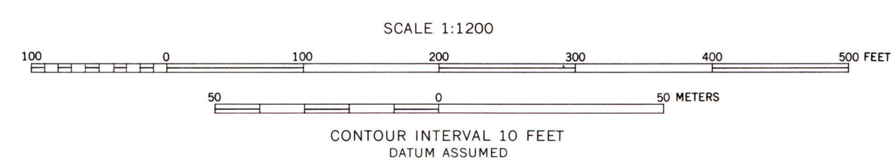
GEOLOGIC MAP OF THE HUNTING HILL SERPENTINITE QUARRY MONTGOMERY COUNTY, MARYLAND
