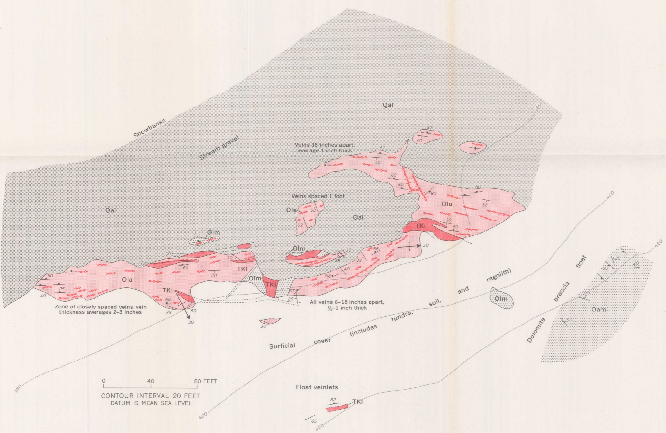
DETAILED MAP ILLUSTRATING THE RELATIONS BETWEEN ORE VEINLETS AND GEOLOGIC STRUCTURES
