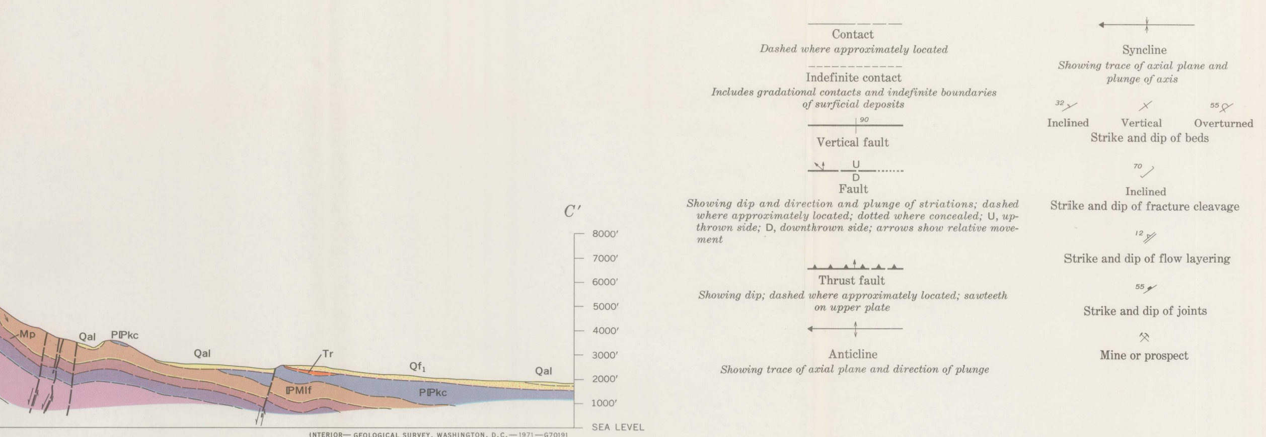
GEOLOGIC MAP AND SECTIONS OF THE PANAMINT BUTTE QUADRANGLE, INYO COUNTY, CALIFORNIA
