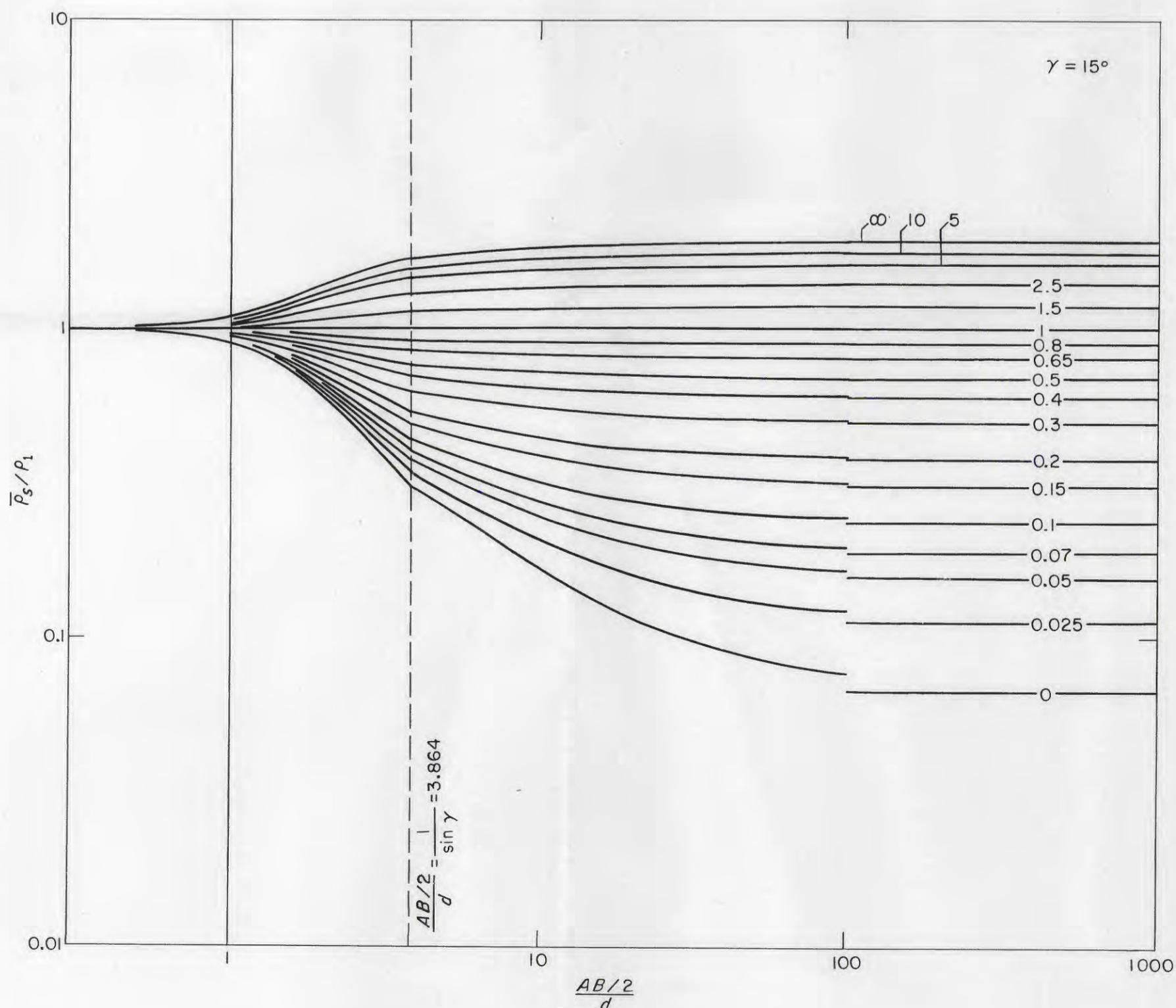
THEORETICAL VES CURVES NEAR A VERTICAL CONTACT FOR VARIOUS VALUES OF RESISTIVITY RATIOS AS A FUNCTION OF THE AZIMUTH ANGLE
