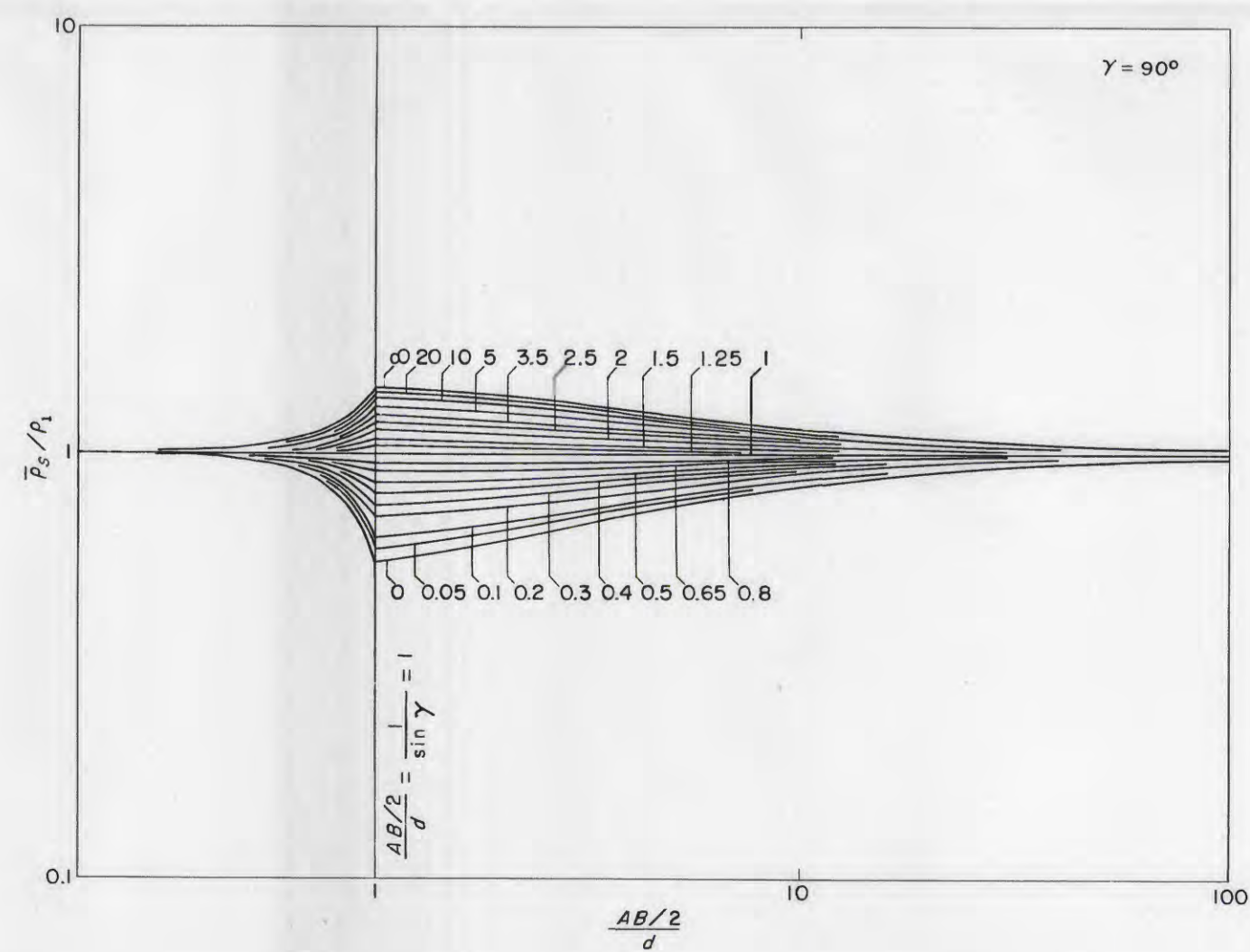
THEORETICAL VES CURVES NEAR A VERTICAL CONTACT FOR VARIOUS VALUES OF RESISTIVITY RATIOS AS A FUNCTION OF THE AZIMUTH ANGLE
