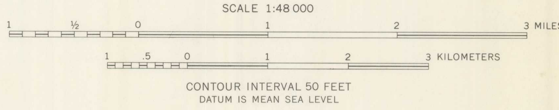
GEOLOGIC AND AEROMAGNETIC MAP OF THE GORE RANGE-EAGLES NEST PRIMITIVE AREA AND VICINITY, EAGLE AND SUMMIT COUNTIES, COLORADO
