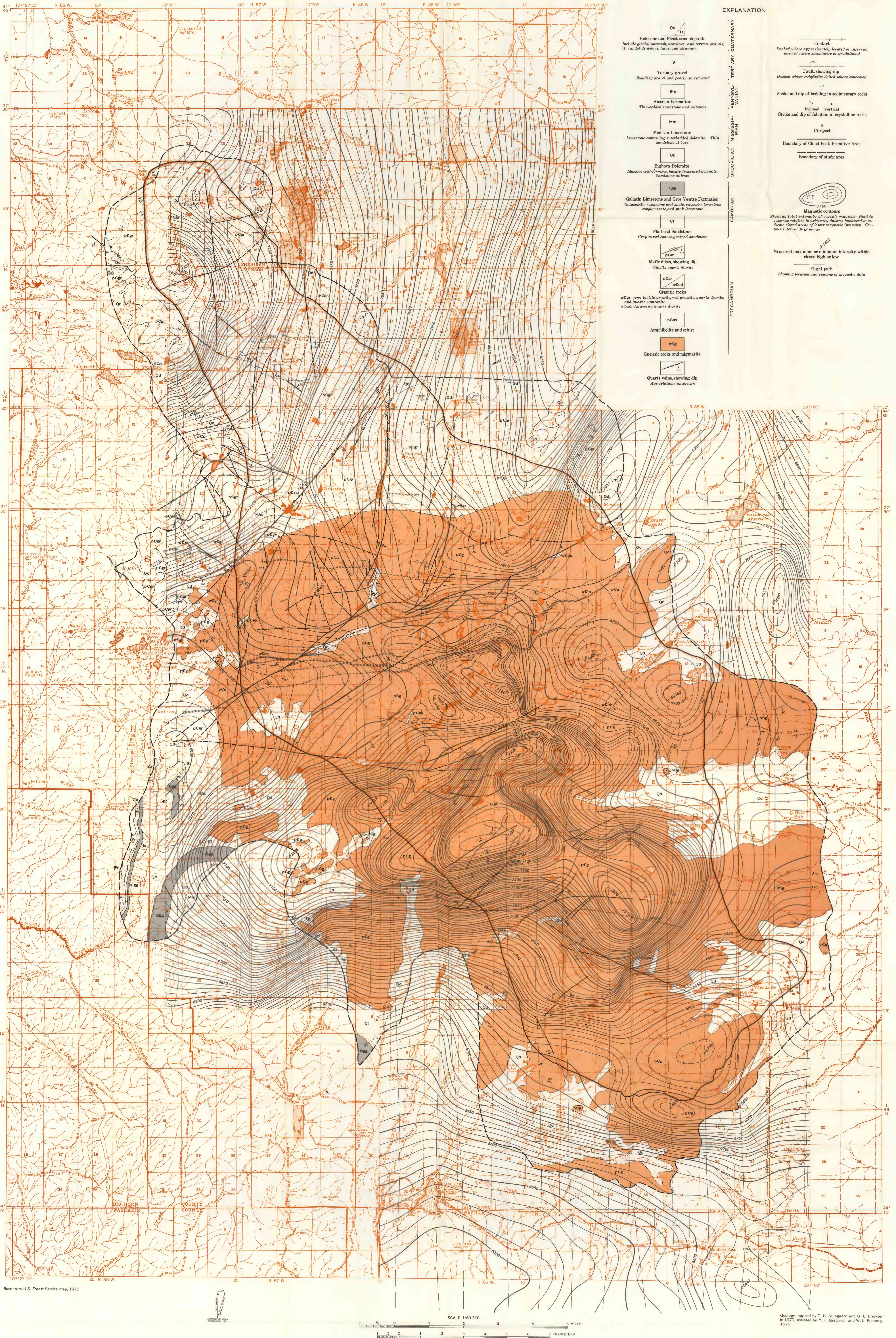
GENERALIZED GEOLOGIC AND MAGNETIC INTENSITY MAP OF THE CLOUD PEAK PRIMITIVE AREA AND VICINITY, WYOMING
