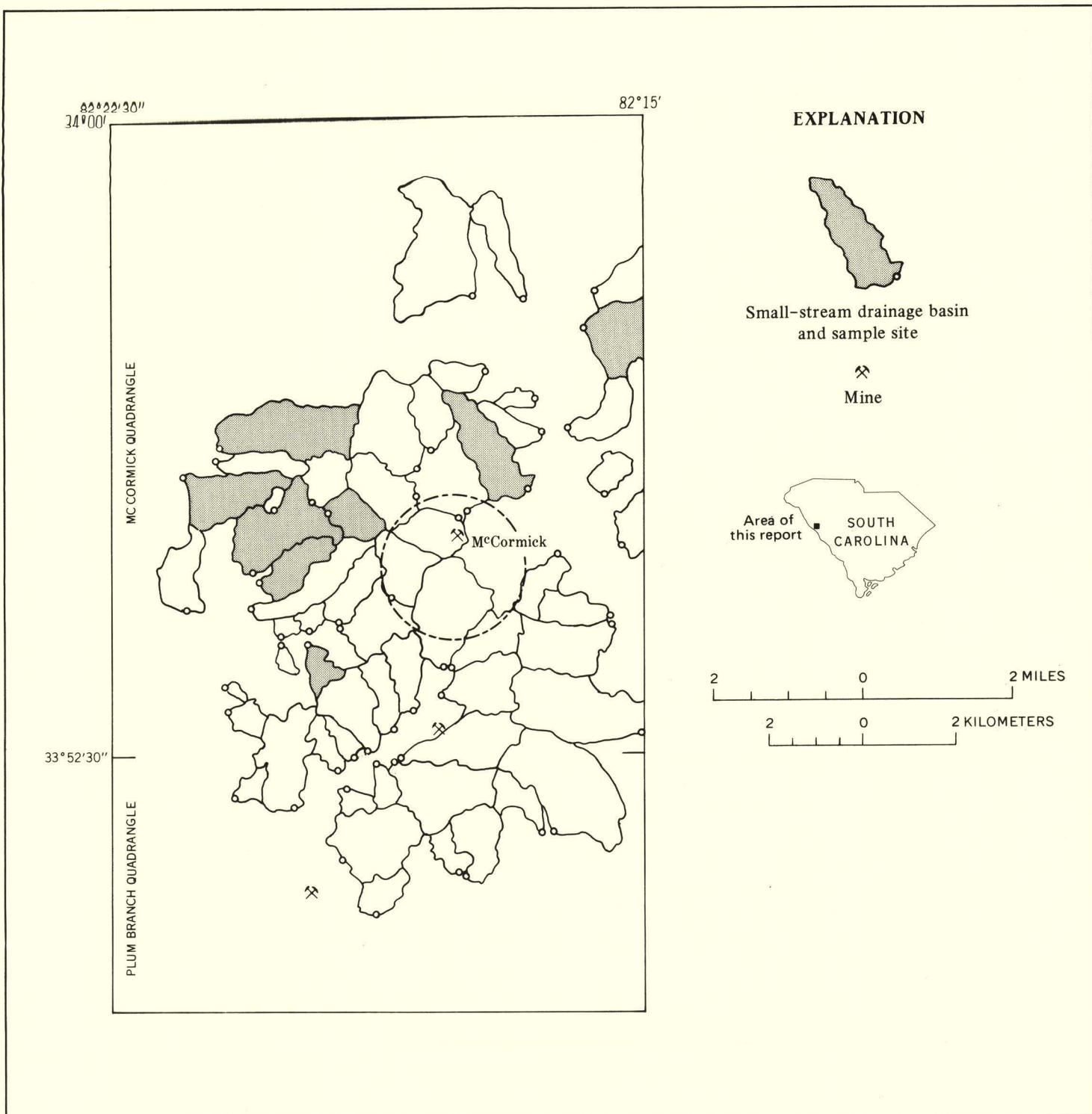
MAP SHOWING SMALL-STREAM DRAINAGE BASINS IN WHICH HEAVY-MINERAL CONCENTRATES CONTAIN A MAGNETIC FRACTION \geq 4.8 GRAMS, MCCORMICK AREA, SOUTH CAROLINA
