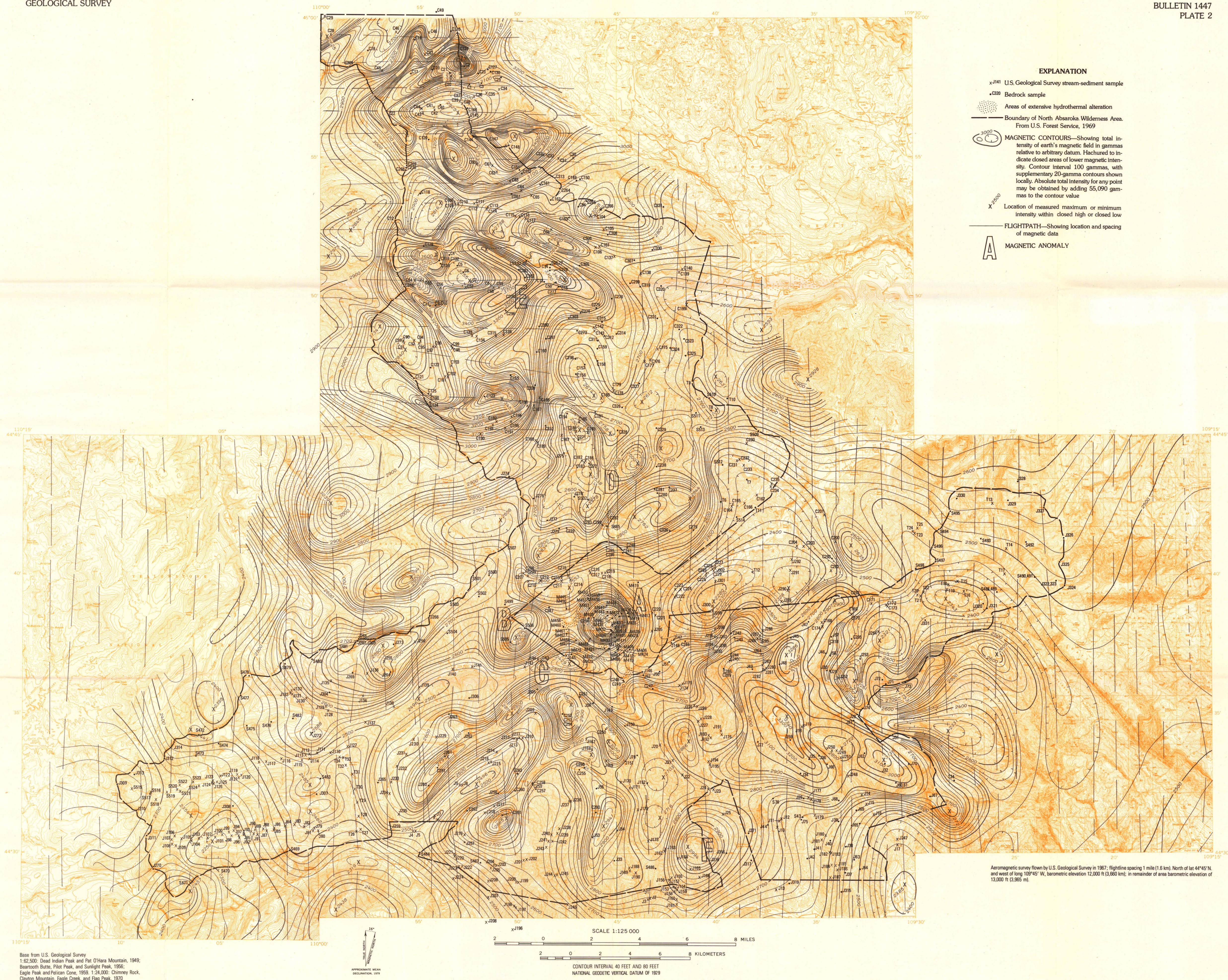
MAP SHOWING AEROMAGNETIC DATA, SAMPLE LOCALITIES, AND ALTERED AREAS, NORTH ABSAROKA WILDERNESS, PARK COUNTY, WYOMING
