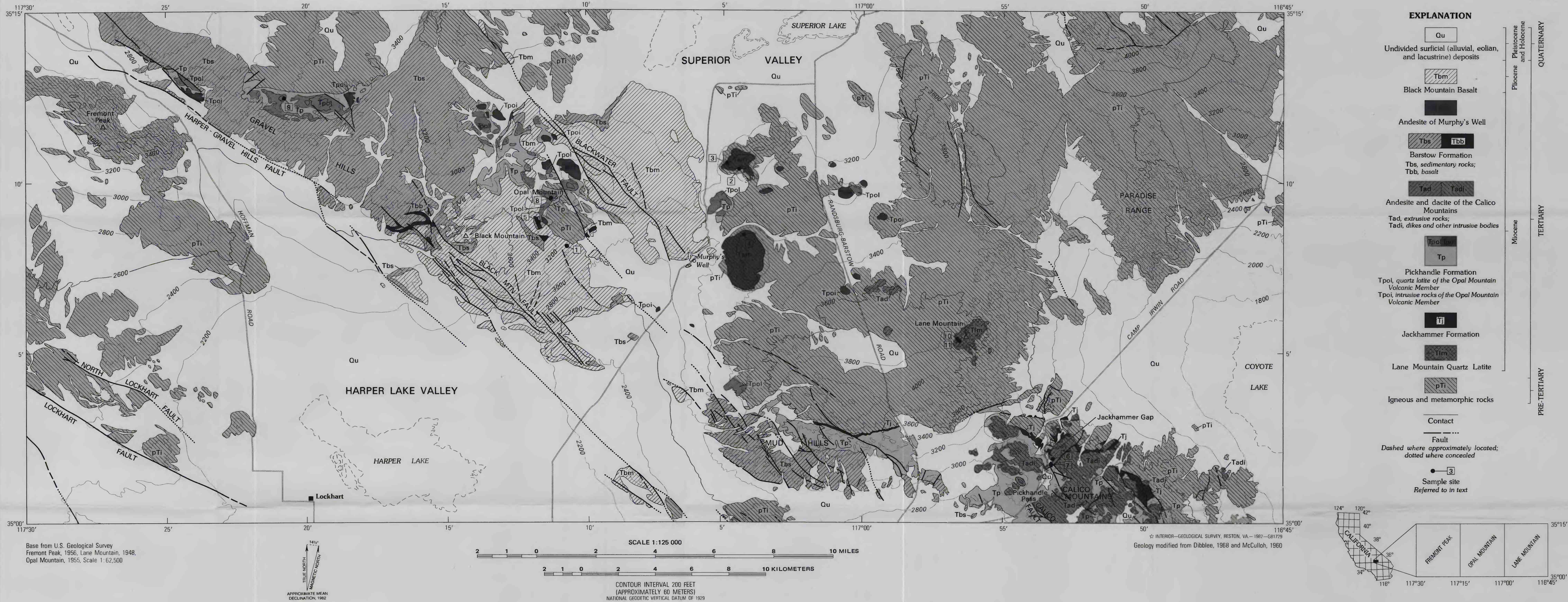
GENERALIZED GEOLOGIC MAP SHOWING POTASSIUM-ARGON AND PALEOMAGNETIC SAMPLE SITES, IN THE BARSTOW BASIN, SOUTHERN CALIFORNIA
