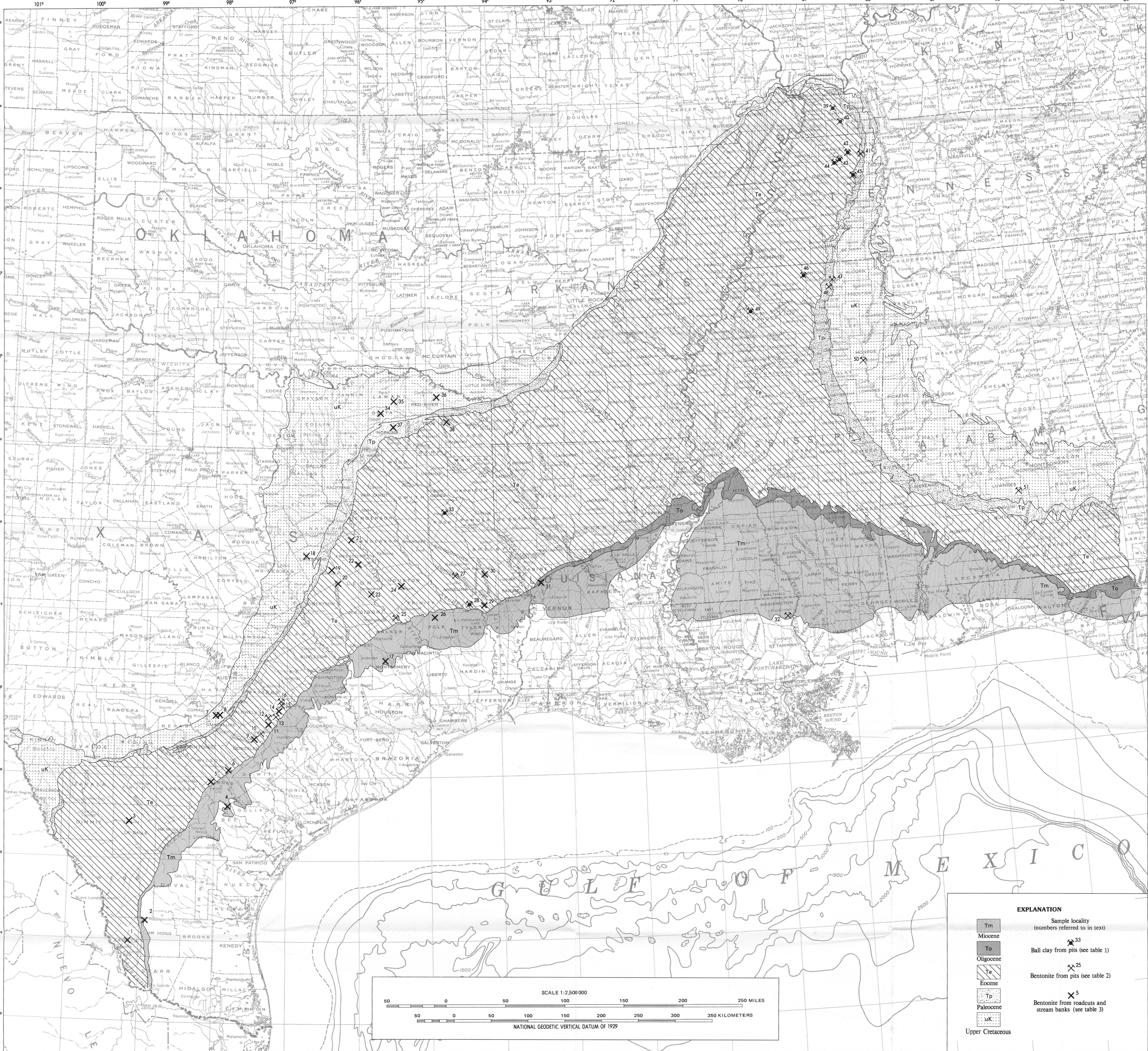
GEOLOGIC MAP OF THE GULF OF MEXICO COASTAL PLAIN, U.S.A.
