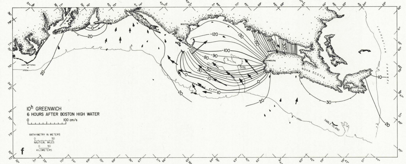
Plate 13. Time sequence of M_2 sea-surface elevation contours and current vectors on the Continental Shelf at two-hour intervals. Sea-level depressions are indicated by tick marks. Current vectors are taken from ellipses in plate 10: a) 0 hr , b) 2 hr , c) 4 hr , d) 6 hr , e) 8 hr , f) 10 hr Greenwich.
