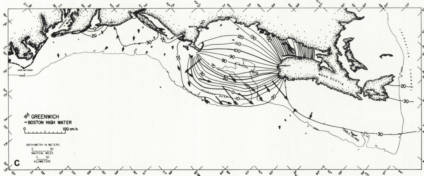
Plate 13. Time sequence of M_2 sea-surface elevation contours and current vectors on the Continental Shelf at two-hour intervals. Sea-level depressions are indicated by tick marks. Current vectors are taken from ellipses in plate 10: a) 0 hr , b) 2 hr , c) 4 hr , d) 6 hr , e) 8 hr , f) 10 hr Greenwich.
