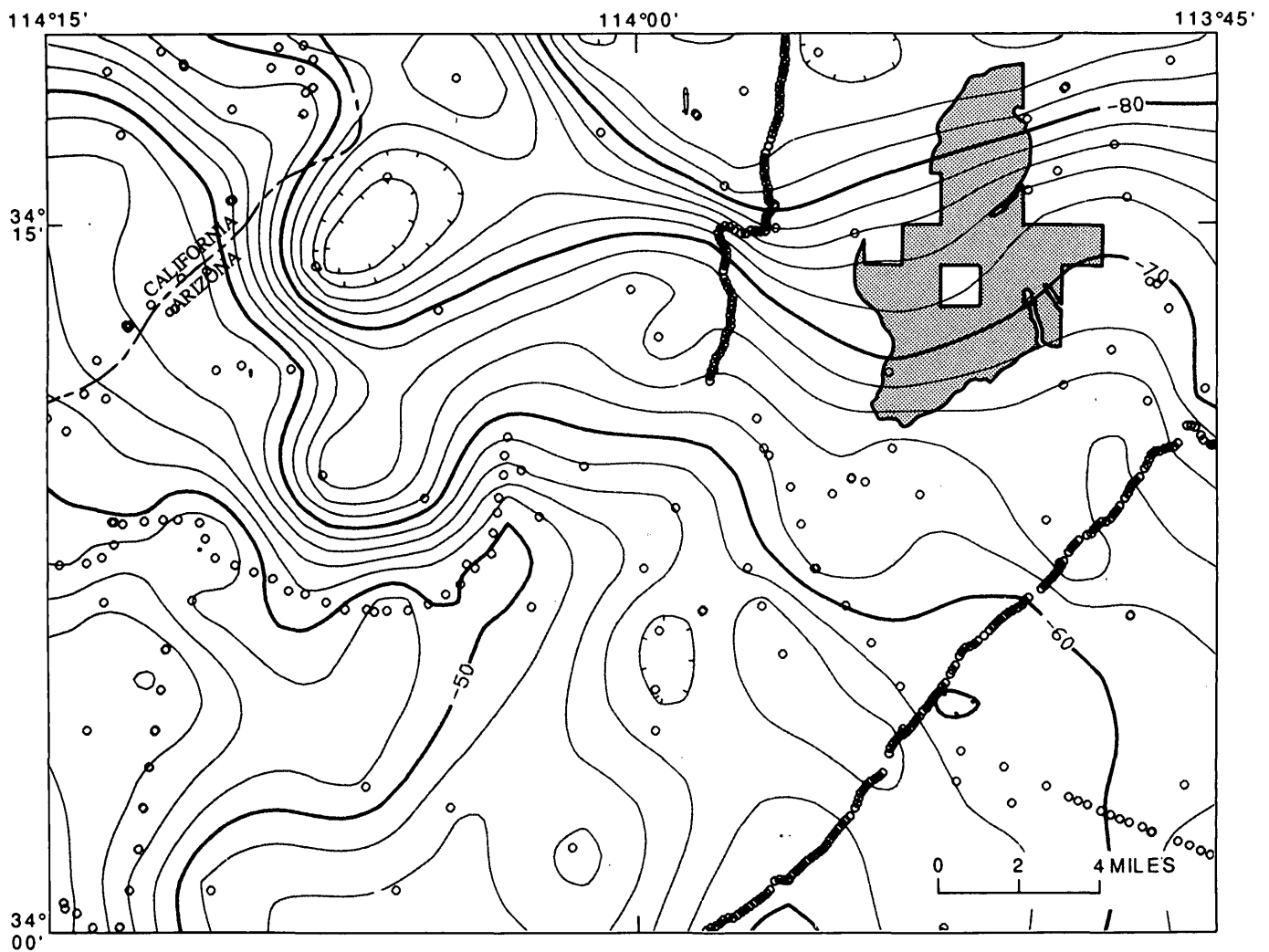
Figure 5. Bouguer gravity anomaly map of the Swansea Wilderness Study Area, La Paz and Mohave Counties, Arizona (shaded). All data reductions and terrane corrections employed a standard Bouguer density of 2.67 g/cm 3 and followed conventional U.S. Geological Survey procedures (for example, Cordell and others, 1982). Contour interval, 2 mGals; hachured in direction of closed low; circle, gravity station.
