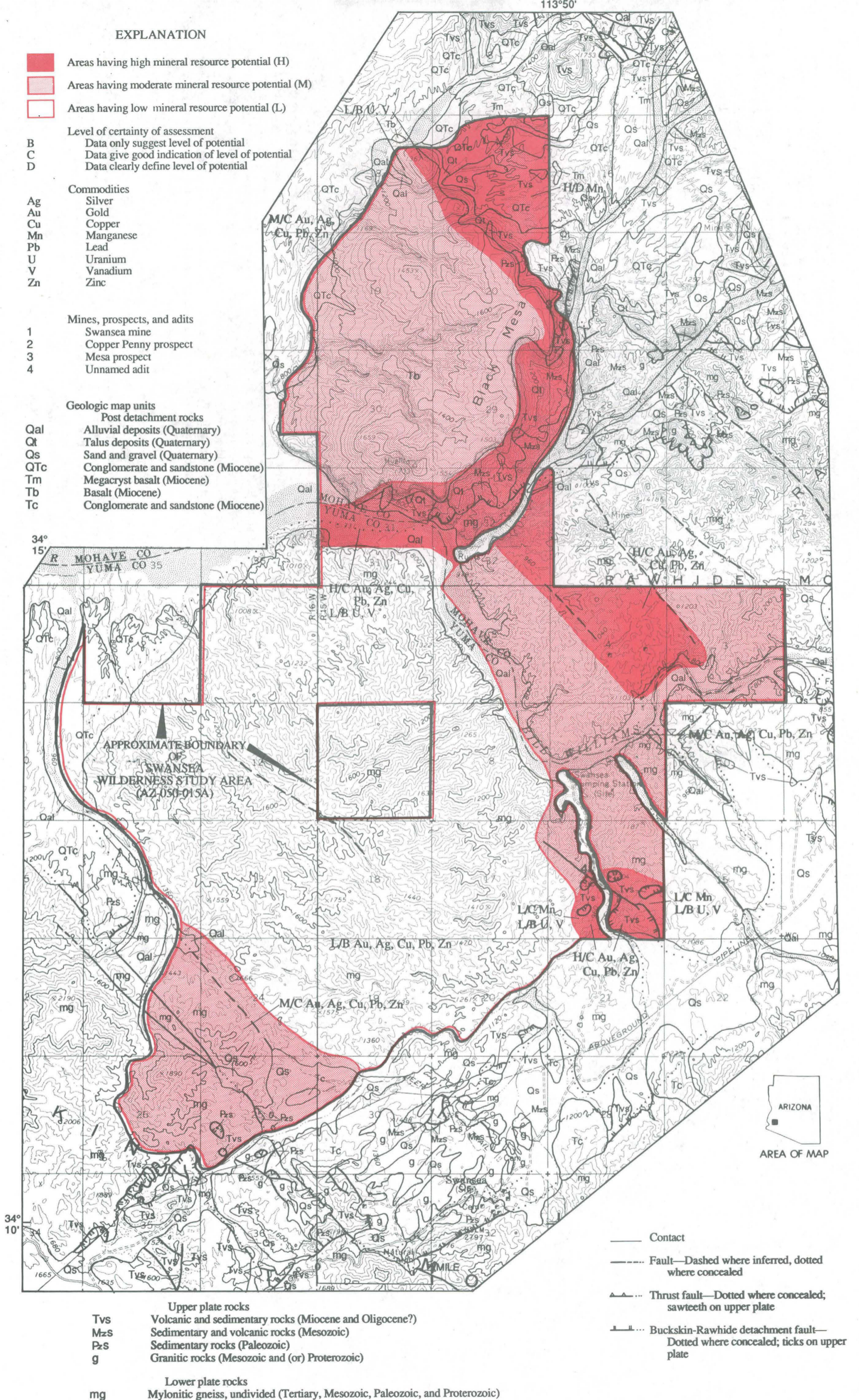
Figure 2. Map showing mineral resource potential and generalized geology of the Swansea Wilderness Study Area, La Paz and Mohave Counties, Arizona. Base from U.S. Geological Survey 1:62,500-scale Swansea and Casteneda Hills quadrangles, 1966. Contour interval 80 ft. Geology north of Bill Williams River is modified from Suneson (1980) and Shackelford (1976, 1989). Geology around Swansea and Copper Penny is modified from Spencer and Reynolds (1987). Geology of rest of area by R.M. Tosdal (1987) and modified from Spencer (1989).
