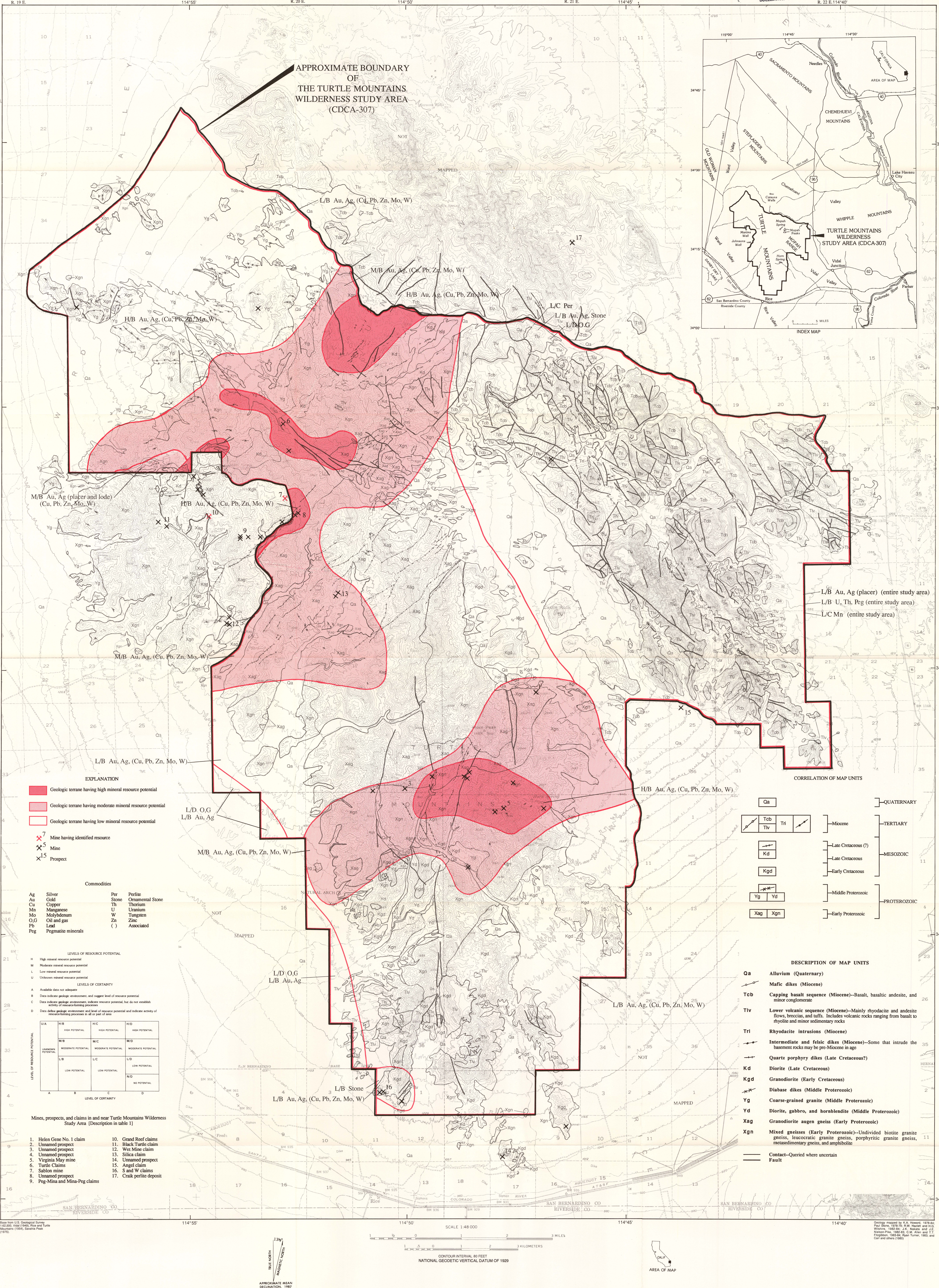
MINERAL RESOURCE POTENTIAL MAP OF THE TURTLE MOUNTAINS WILDERNESS STUDY AREA, SAN BERNARDINO COUNTY, CALIFORNIA
