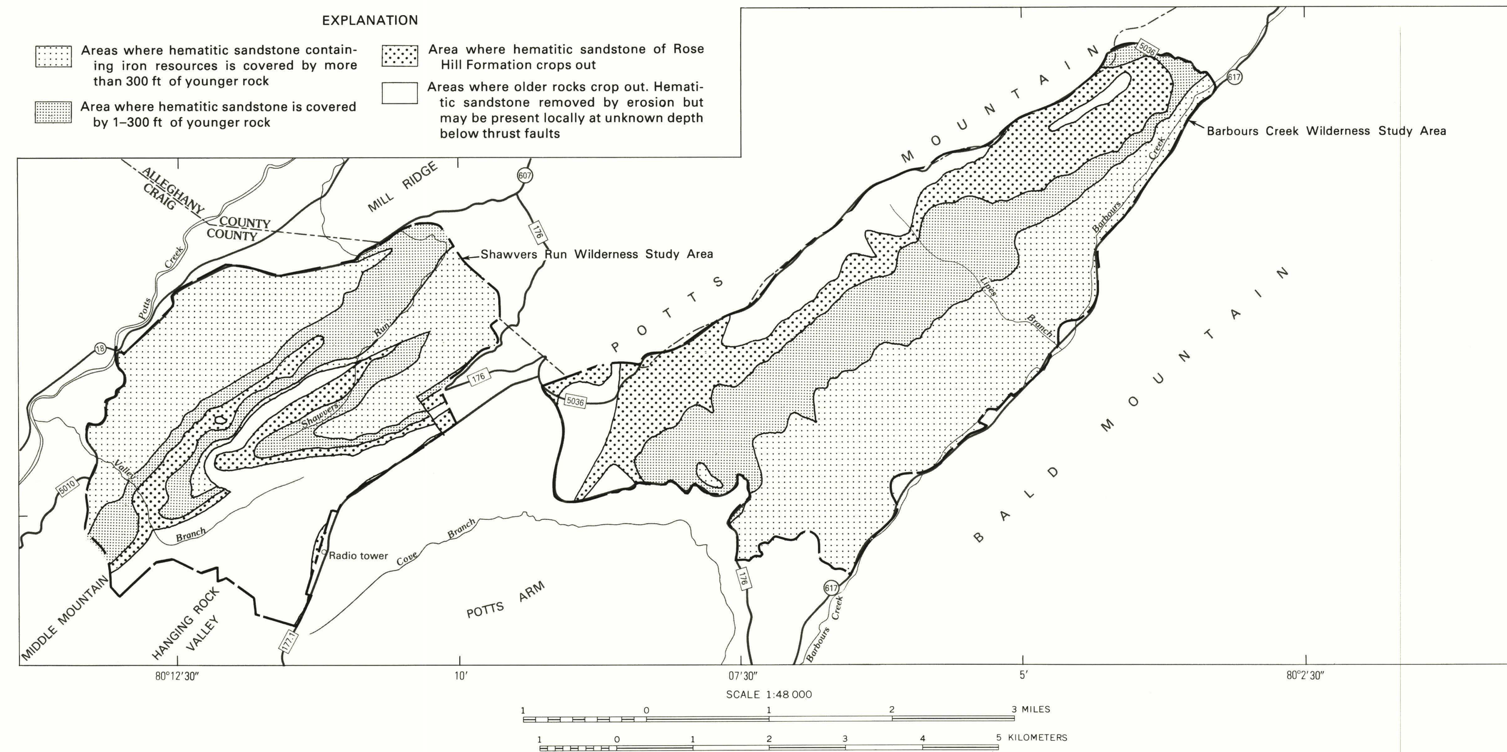
B. MAP SHOWING DISTRIBUTION OF INFERRED SUBECONOMIC HEMATITIC IRON RESOURCES
