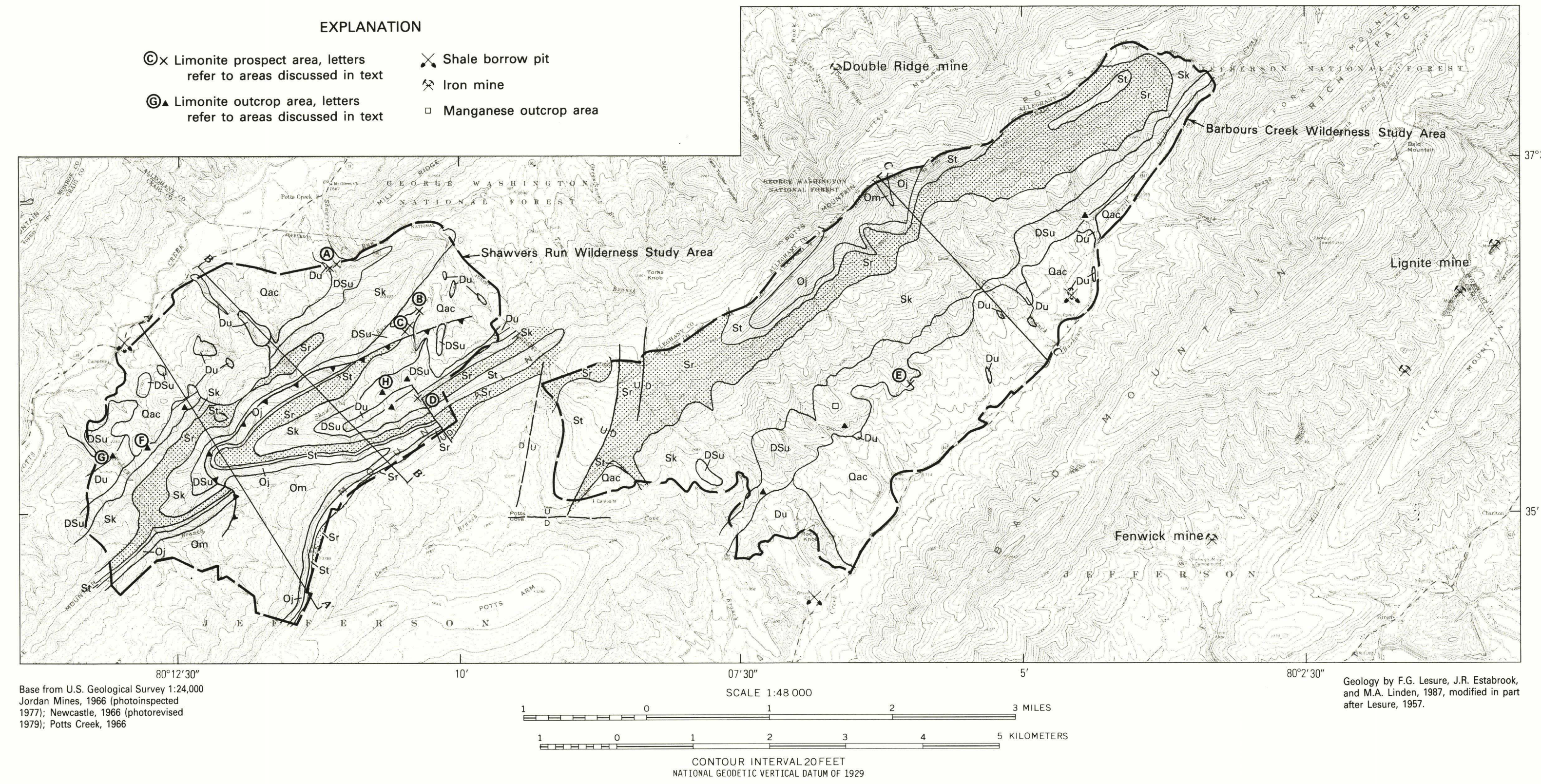
A. GEOLOGIC MAP AND CROSS SECTIONS SHOWING LIMONITE OUTCROP AREAS
