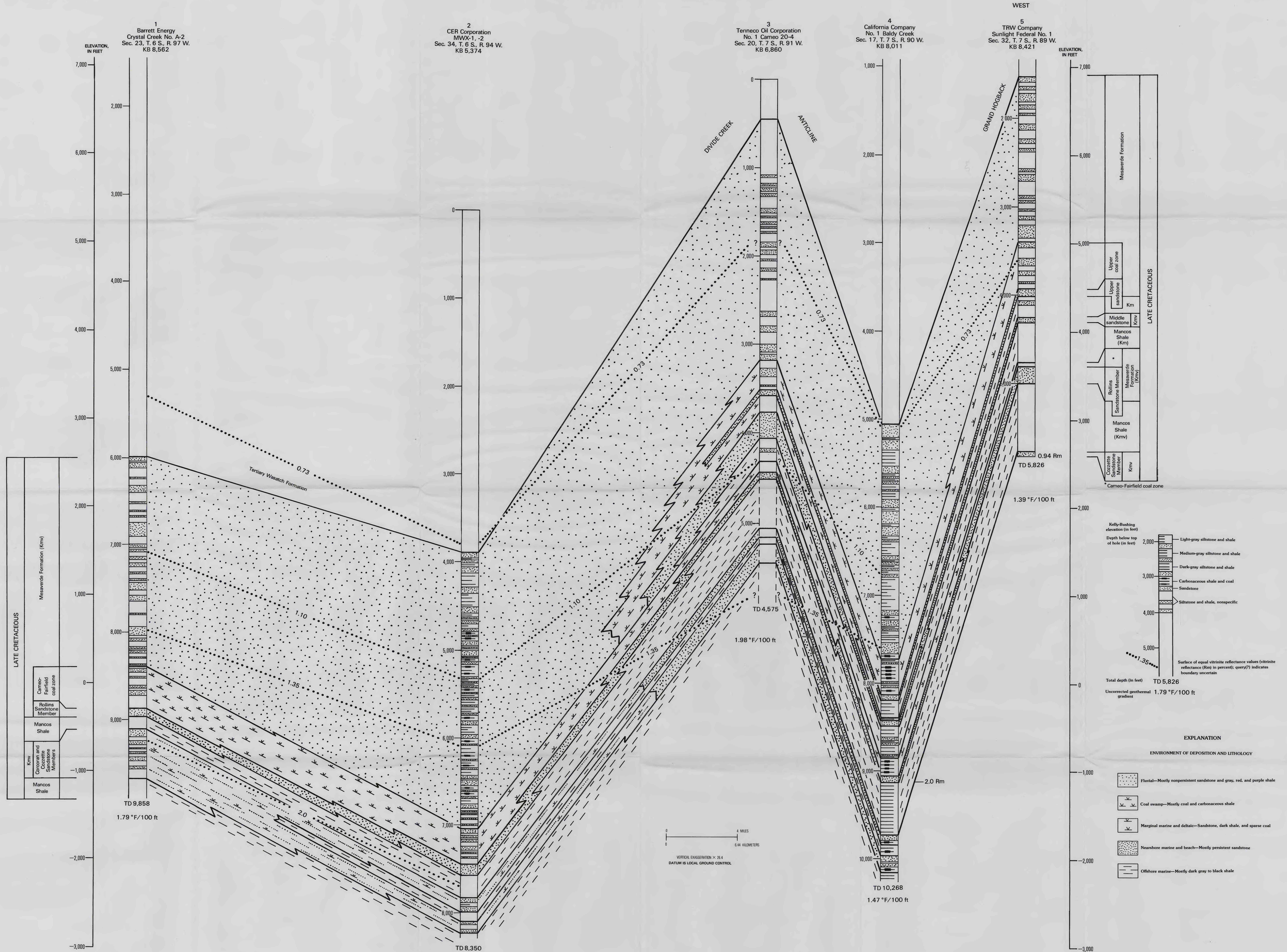
CROSS SECTION OF CRETACEOUS MANCOS SHALE AND MESAVERDE FORMATION SHOWING STRUCTURE, STRATIGRAPHY, AND THERMAL MATURITY, PICEANCE BASIN, NORTHWESTERN COLORADO
