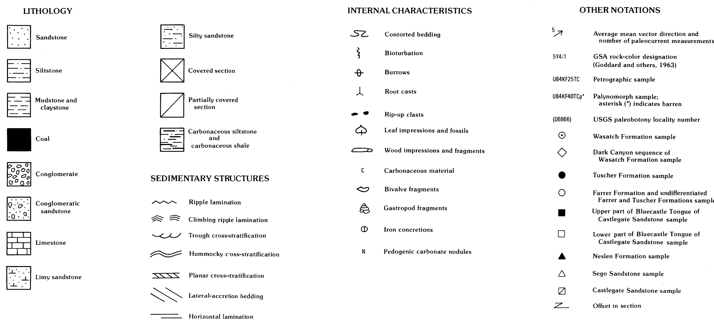
Tusher Canyon Type section for Farrer and Tusher Formations Sec. 9, 16, 13, T. 20 S., R. 17 E.; sec. 1, T. 20 S., R. 18 E.; sec. 19, T. 19 S., R. 19 E.
