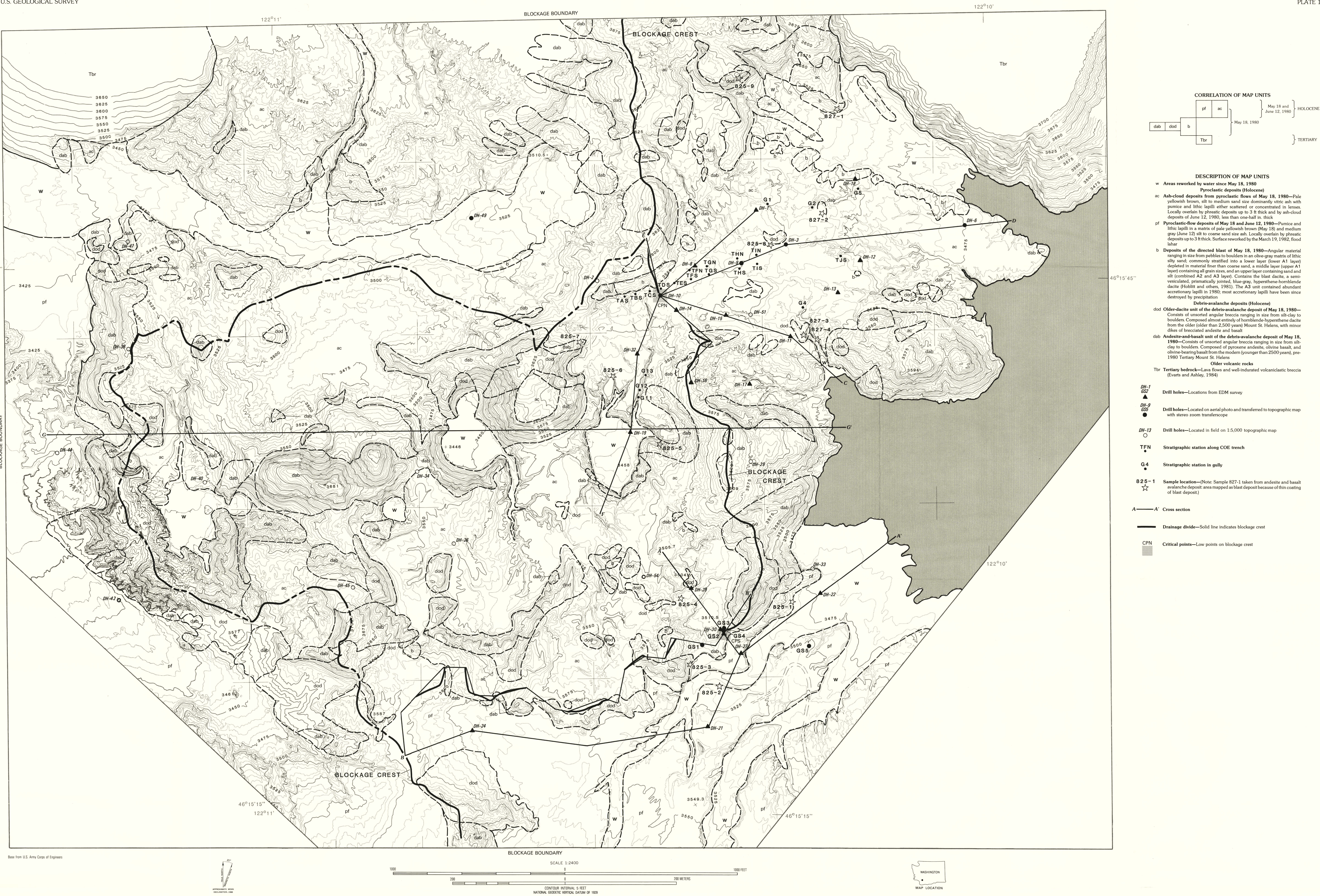
GEOLOGIC MAP OF SPIRIT LAKE BLOCKAGE, SHOWING LOCATIONS OF DRILL HOLES, DRAINAGE DIVIDES, AND CRITICAL POINTS RELATIVE TO POTENTIAL LAKE BREAKOUT
