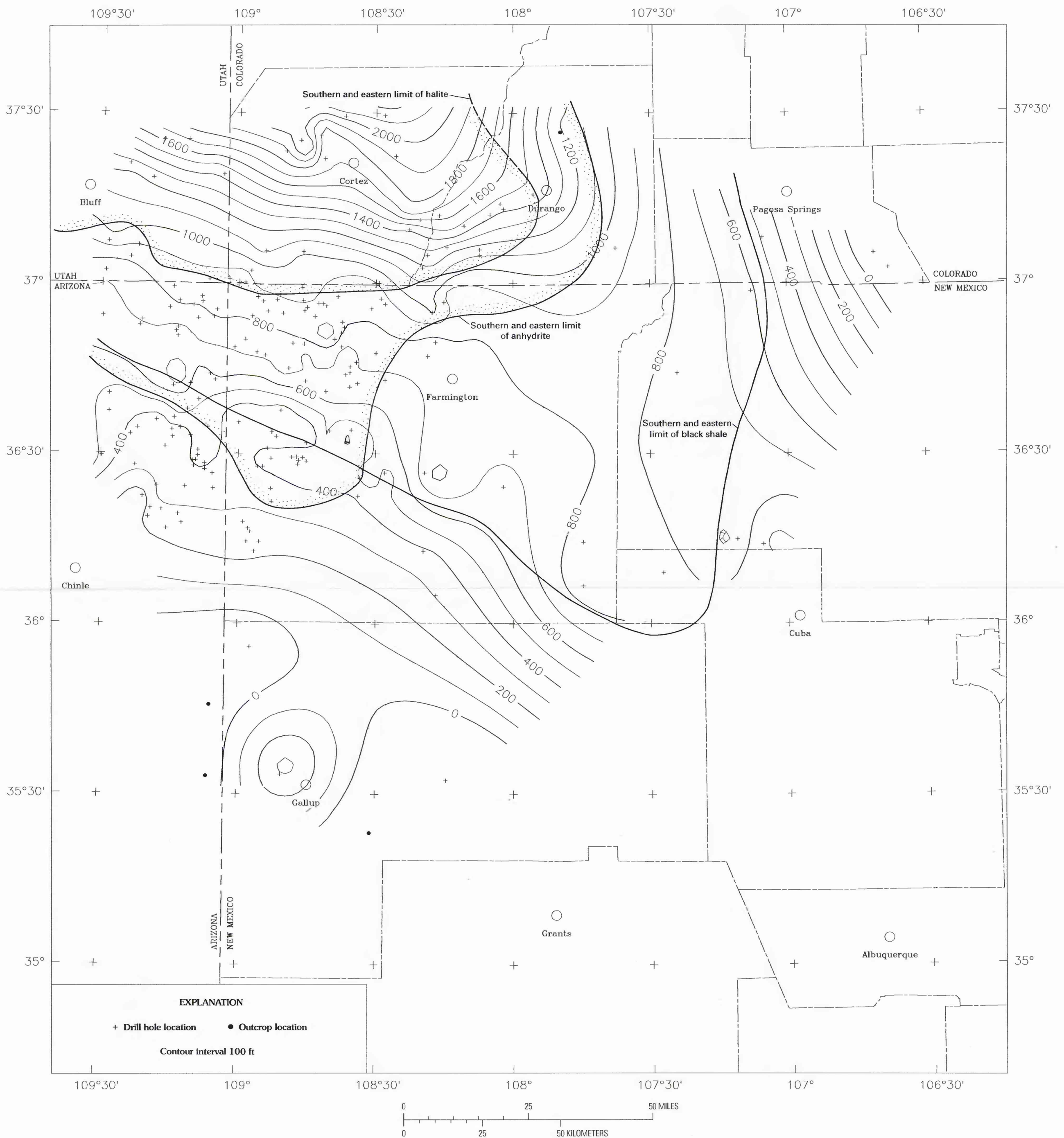
MAP SHOWING THICKNESS OF THE PARADOX FORMATION AND RELATED ROCKS, SAN JUAN BASIN AND ADJACENT AREAS, UTAH, COLORADO, ARIZONA, AND NEW MEXICO
