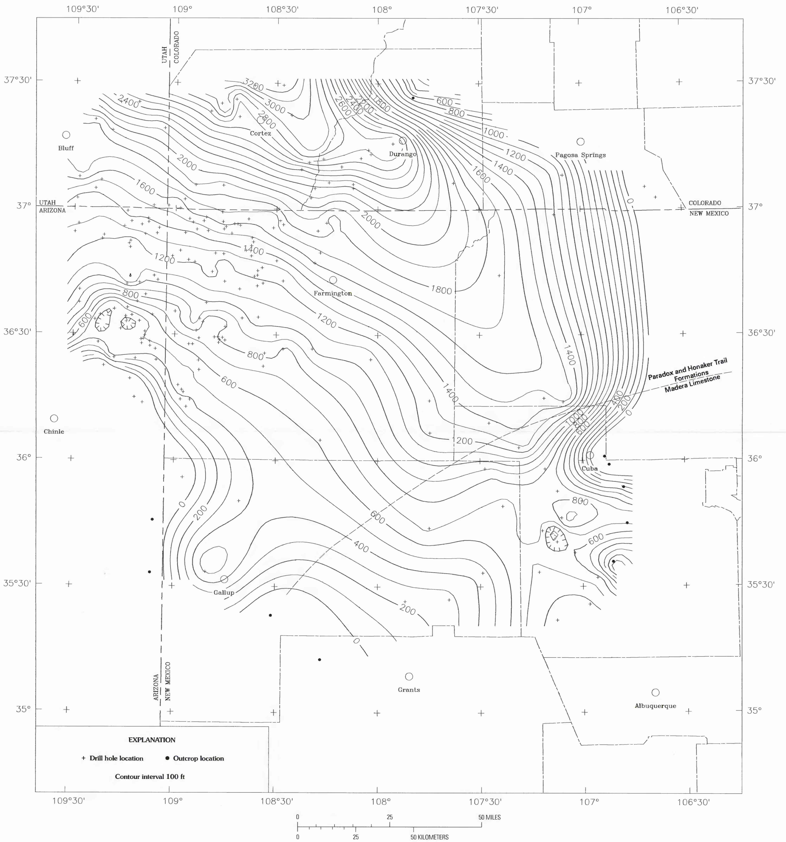
MAP SHOWING THICKNESS OF THE COMBINED PARADOX AND HONAKER TRAIL FORMATIONS AND THE MADERA LIMESTONE, SAN JUAN BASIN AND ADJACENT AREAS, UTAH, COLORADO, ARIZONA, AND NEW MEXICO
