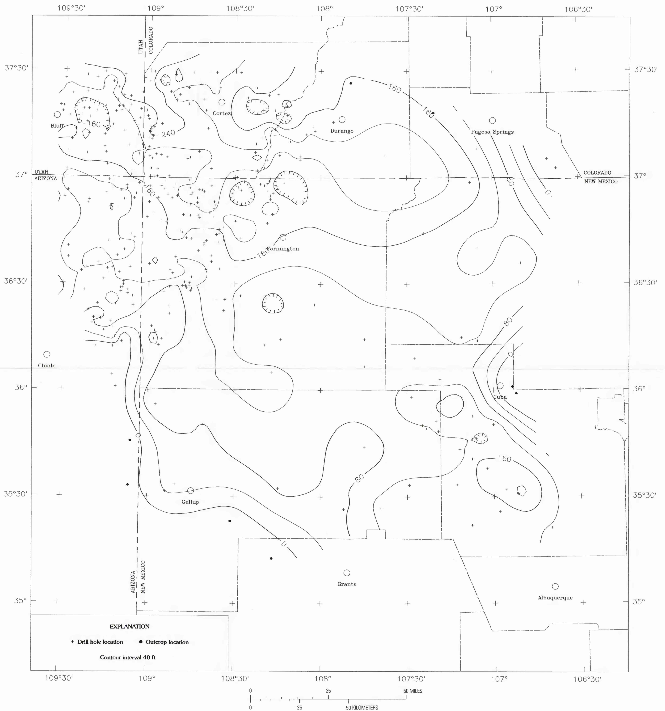
MAP SHOWING THICKNESS OF THE RICO FORMATION, SAN JUAN BASIN AND ADJACENT AREAS, UTAH, COLORADO, ARIZONA, AND NEW MEXICO
