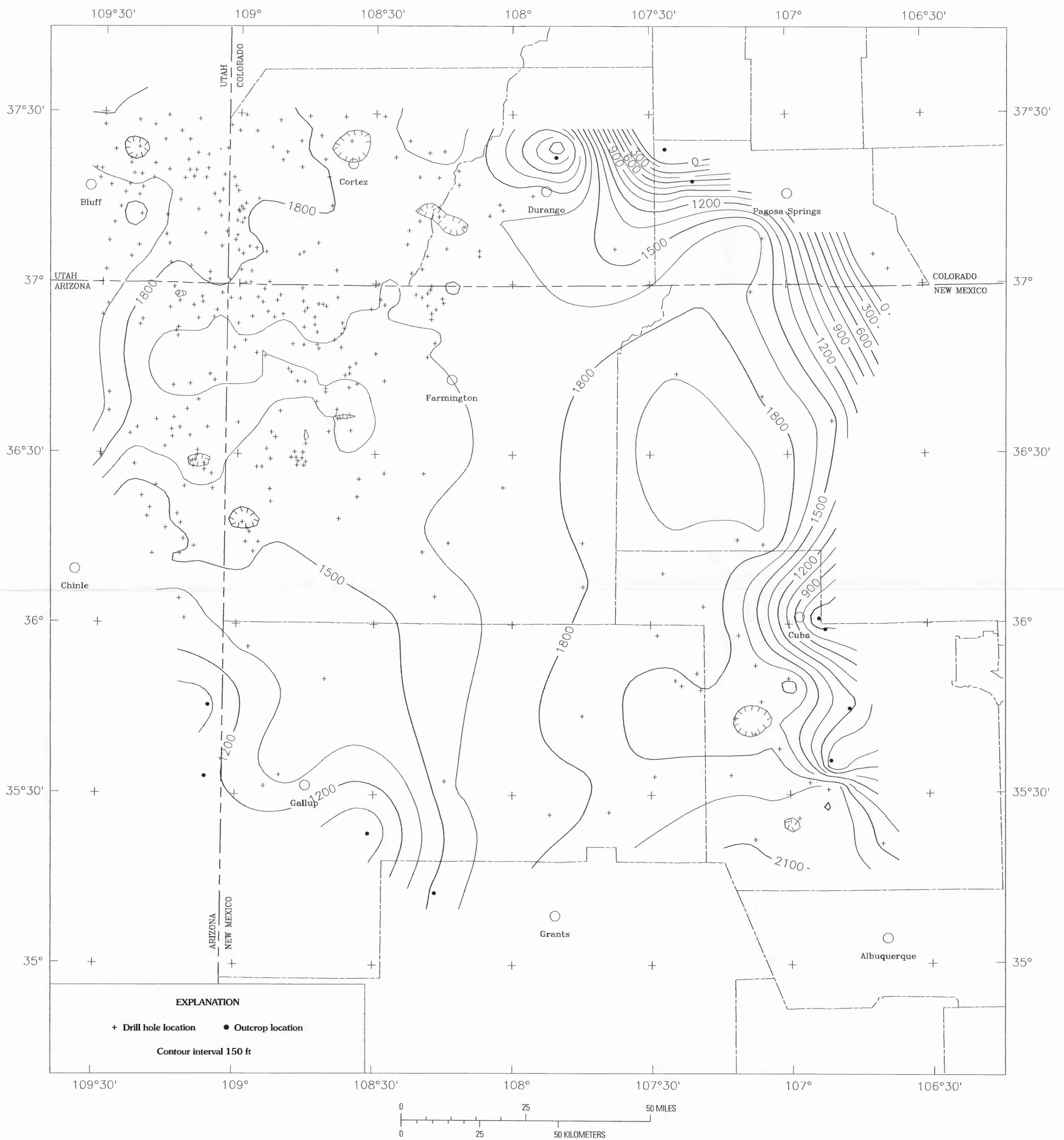
MAP SHOWING THICKNESS OF ALL PERMIAN ROCKS, SAN JUAN BASIN AND ADJACENT AREAS, UTAH, COLORADO, ARIZONA, AND NEW MEXICO
