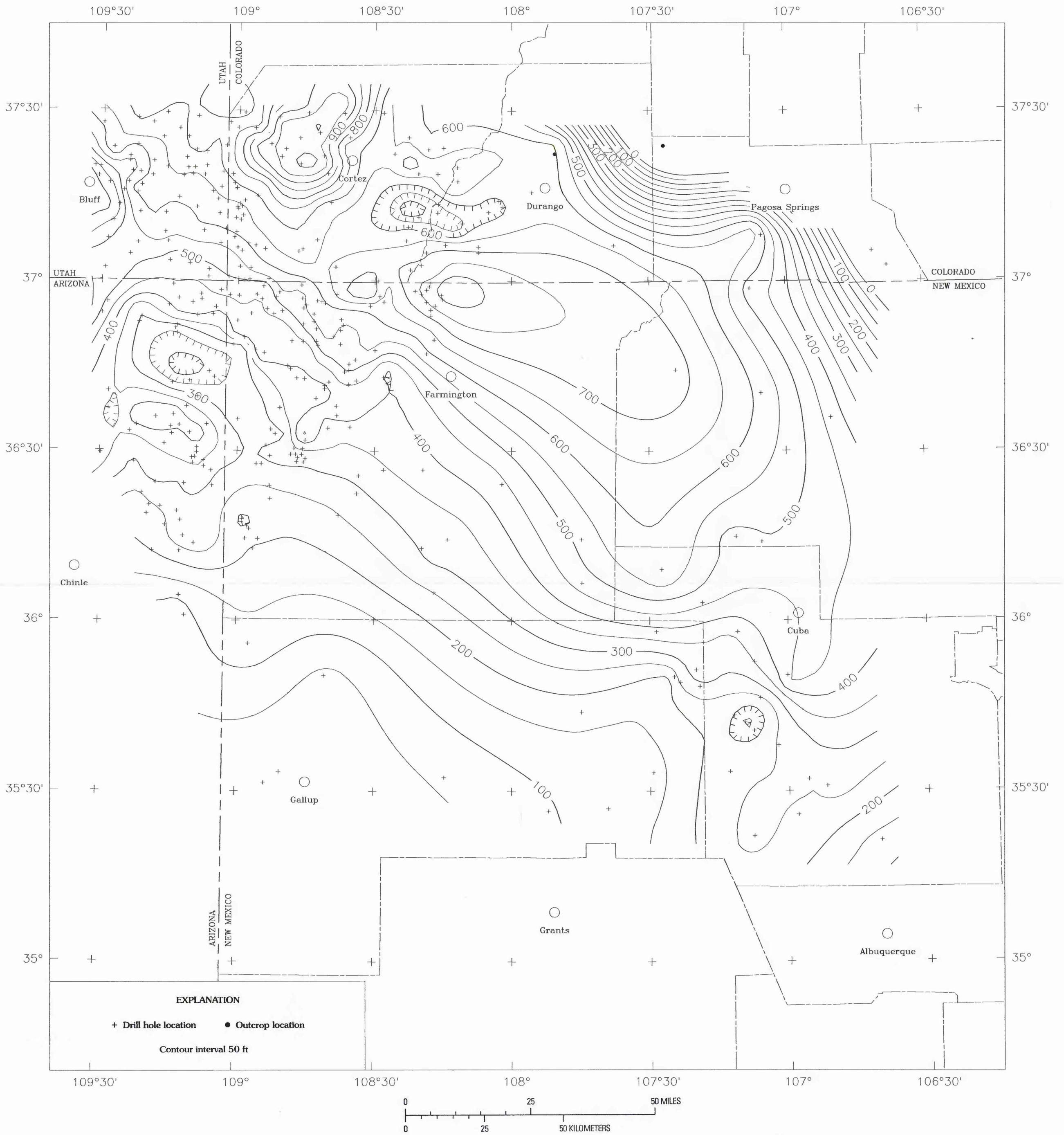
MAP SHOWING THICKNESS OF THE HALGAITO FORMATION AND RELATED ROCKS, SAN JUAN BASIN AND ADJACENT AREAS, UTAH, COLORADO, ARIZONA, AND NEW MEXICO
