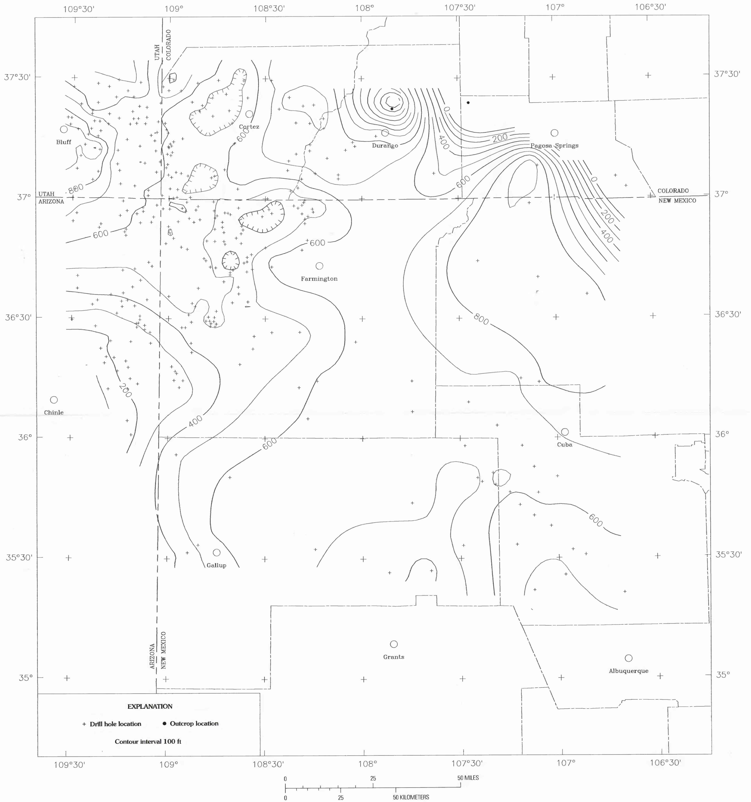
MAP SHOWING THICKNESS OF THE ORGAN ROCK FORMATION AND RELATED ROCKS, SAN JUAN BASIN AND ADJACENT AREAS, UTAH, COLORADO, ARIZONA, AND NEW MEXICO
