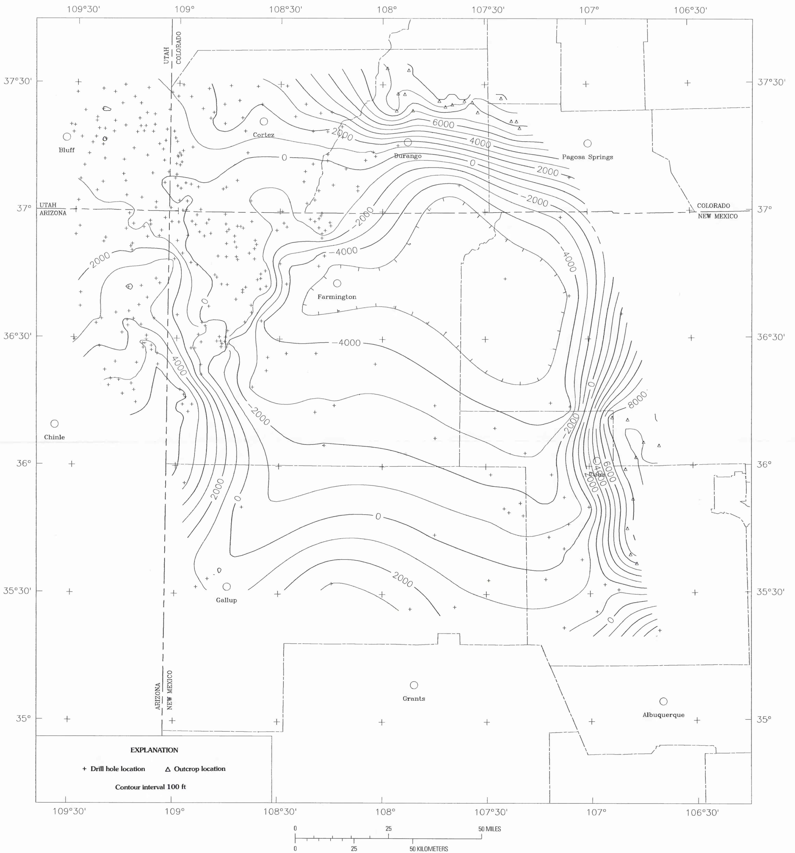
MAP SHOWING STRUCTURE CONTOURS DRAWN ON THE TOP OF THE RICO FORMATION, SAN JUAN BASIN AND ADJACENT AREAS, UTAH, COLORADO, ARIZONA, AND NEW MEXICO
