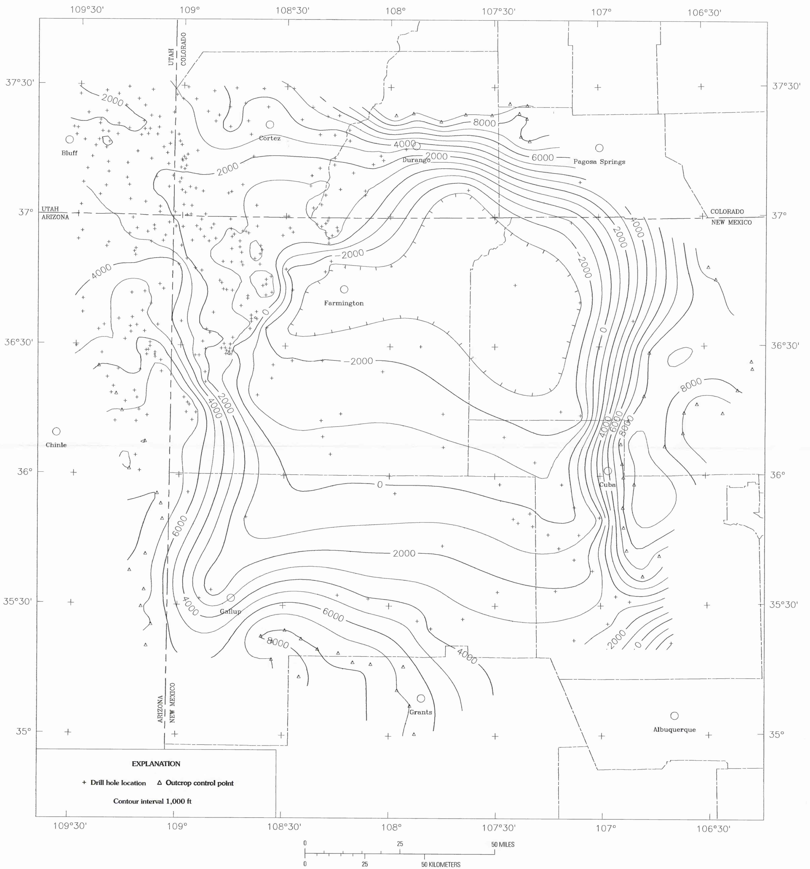
MAP SHOWING STRUCTURE CONTOURS DRAWN ON THE TOP OF THE PERMIAN SYSTEM, SAN JUAN BASIN AND ADJACENT AREAS, UTAH, COLORADO, ARIZONA, AND NEW MEXICO
