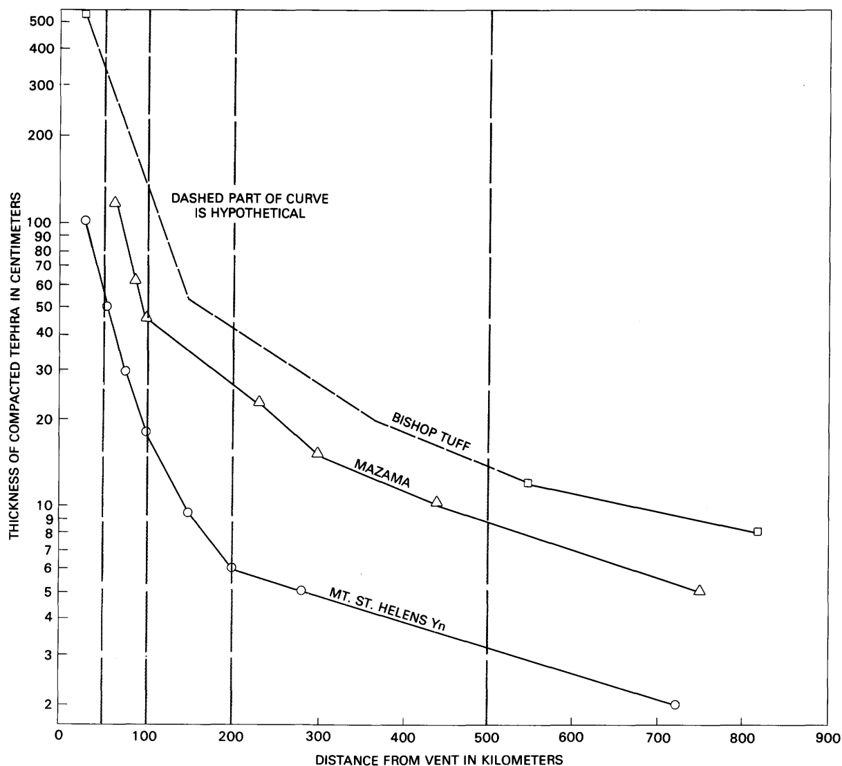
Figure 3. Plot of ash thickness versus distance for compacted ash falls from large (several cubic kilometers) to very large (hundreds of cubic kilometers) eruptions of three different sizes. Data based on individual eruptions of Mount St. Helens (volume about 3 km 3 ), Mount Mazama (volume about 40 km 3 ), and Bishop Tuff (volume about 600 km 3 ). Data from this figure can be compared with figure 2 to estimate possible locations and compacted thicknesses of future ash falls from large to very large eruptions in California. Data on Mount St. Helens eruption from Mullineaux, 1977; D. R. Mullineaux, written commun., 1985; Westgate and Dreimanis, 1967. Data on Mount Mazama eruption from Williams and Gole, 1968; Rai, 1971; and Mehringer and others, 1977. Data on Bishop Tuff eruption from Izett, 1982; and unpublished data of the authors.
