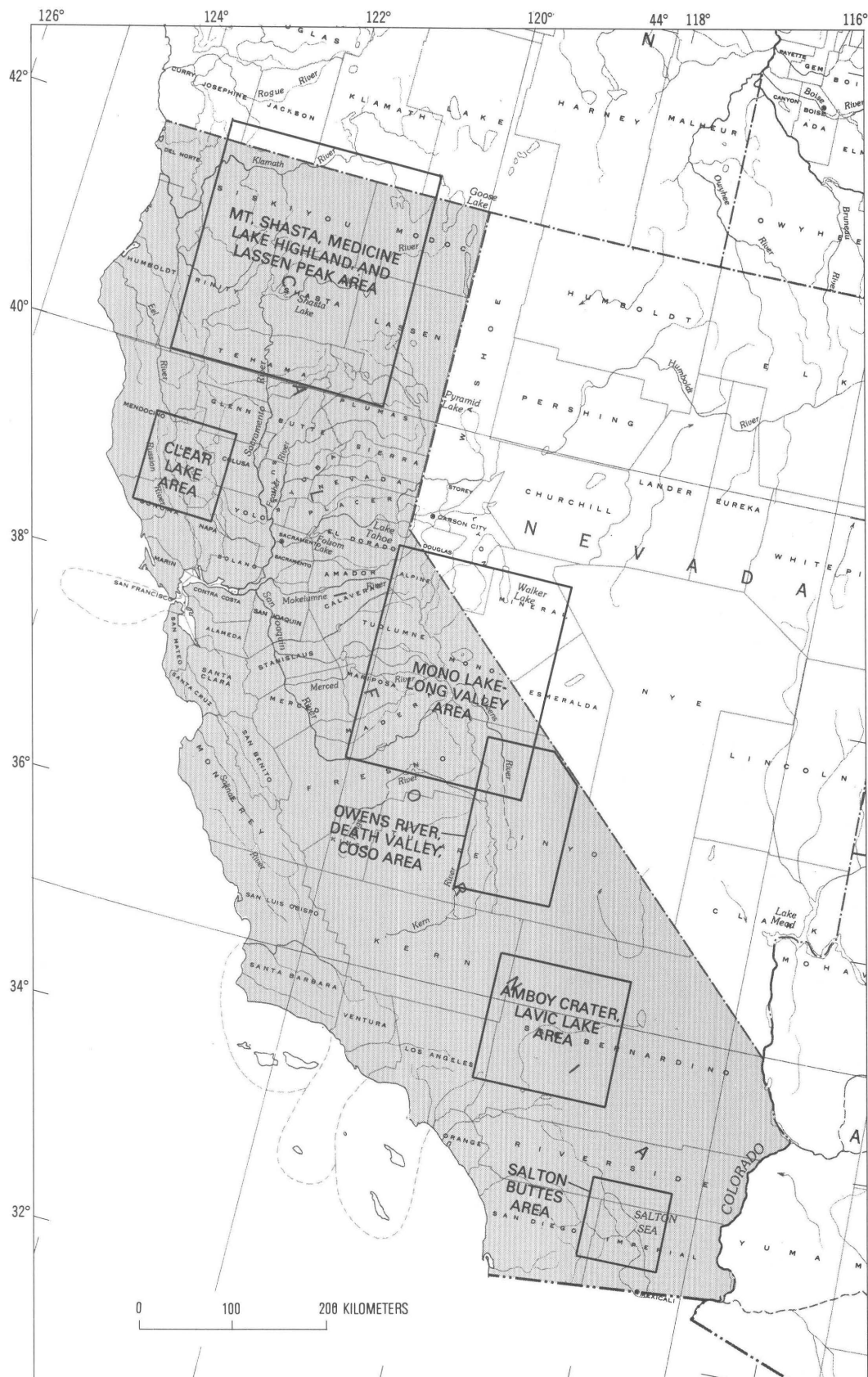
Figure 1. Areas subject to potential hazards from future eruptions in California. Areas numbered I to VI are shown in detail as separate illustrations on plate 1.
